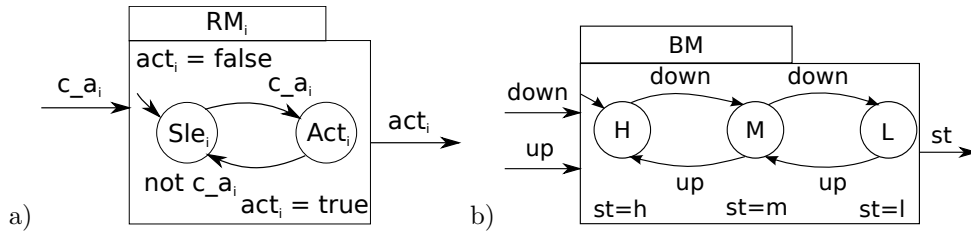
Figure 5.4: Models RM_i for tile A_i , and BM for battery.
