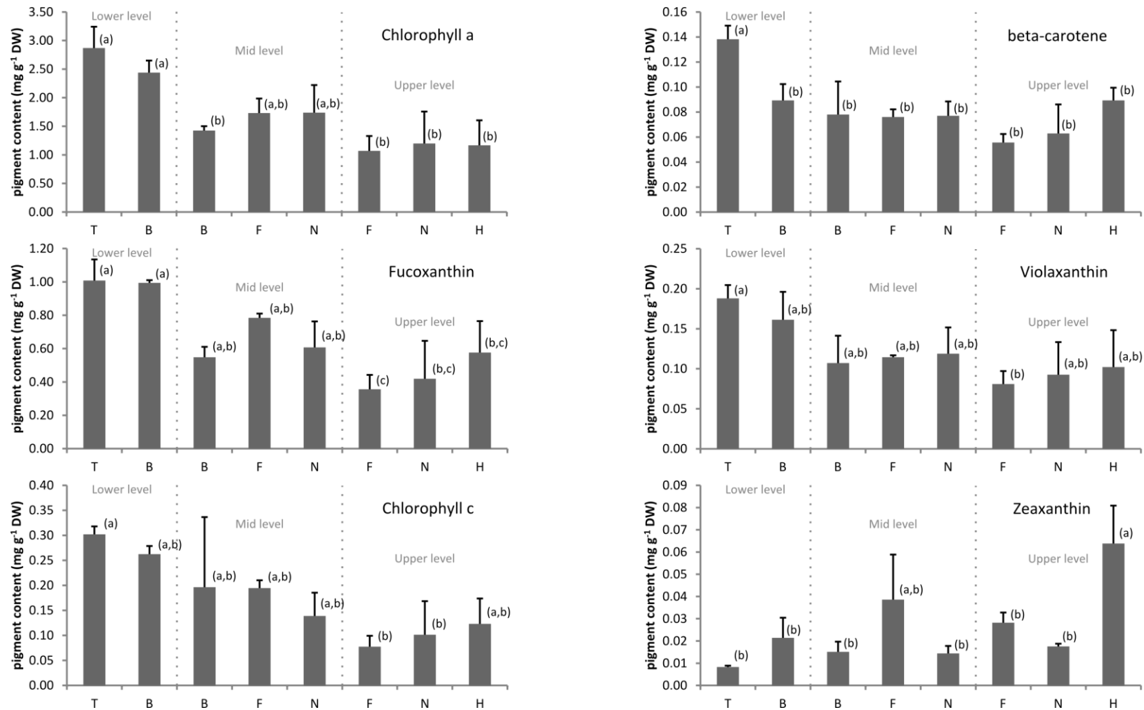
Figure 2: pigments contents in Cystoseira species from Brittany (France) according to their position on the shore. Cystoseira baccata “B”, C. fœniculacea “F”, C. humilis “H”, C. nodicaulis “N” and C. tamariscifolia “T”. For each pigment analysis, values sharing a common letter in parentheses were not statistically different according to Tukey’s HSD test. The scale for each graph is not similar.
