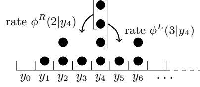
Figure 3.5: Rates of two possible transitions in the q -Hahn asymmetric zero-range process.
