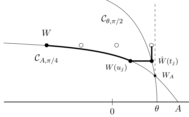
Figure 2.6: The thick line is the path from W to W + j with j = 3 in the case 2 : \Re[q^{W+j}] < q^\theta and \Re[W + j] \leq \Re[W_A] .
