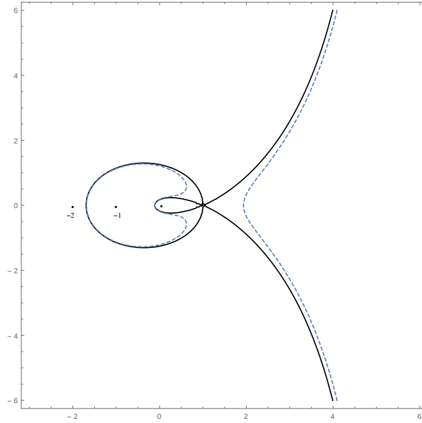
Figure 4.8: The solid lines are contour lines \Re\mathfrak{e}[H(z)] = \Re\mathfrak{e}[H(\theta)] in the case \theta = a = b = 1 . Dashed lines are contour lines \Re\mathfrak{e}[H(z)] = \Re\mathfrak{e}[H(\theta)] + 2\eta with \eta = 0.05 .
