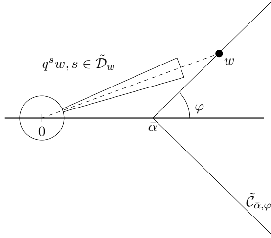
Figure 2.2: The contours in Definition 2.2.1. One sees that q^s w, s \in \tilde{\mathcal{D}}_w stays to the left of \tilde{\mathcal{C}}_{\bar{\alpha}, \varphi} .
