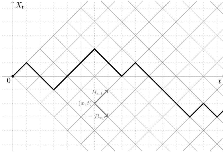
Figure 4.1: The graph of t \mapsto X_t for the Beta RWRE. One sees that that the random walk \mathbf{X}_t := (t, X_t) is also a (directed) random walk in a random environment in \mathbb{Z}^2 .
