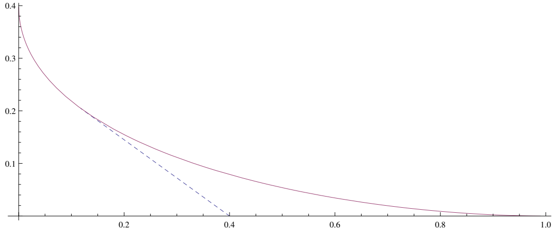
Figure 2.1: Limit shapes of \frac{1}{\tau}(X_N(\tau) + N, N) for q = 0.6 . The solid line corresponds to \alpha = 1 (no slow particle). The dashed line corresponds to \alpha = 0.4 (one or several slower particles). Note that the curved line is the parametric curve (f/\kappa, 1/\kappa) , whereas the straight line part is the parametric curve (g/\kappa, 1/\kappa) , when \theta ranges from 0 to \log_q \alpha , i.e. \theta satisfying the condition \alpha < q^\theta .
