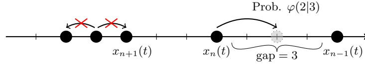
Figure 3.4: Jumps probabilities in the (discrete-time) q -Hahn TASEP.
