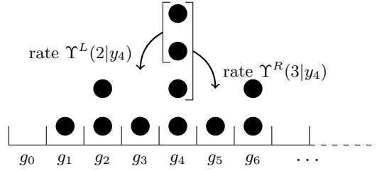
Figure 1.10: A general zero-range process.
