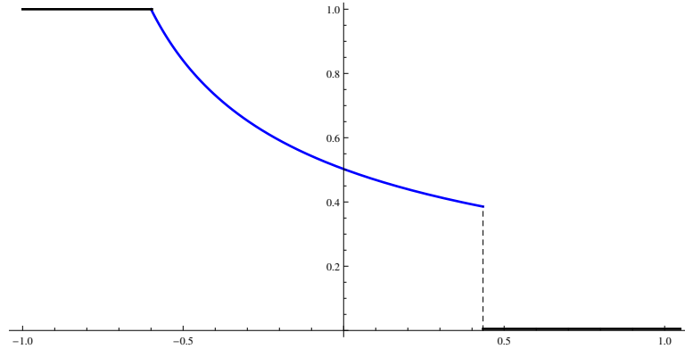
Figure 3.3: Density profile x \mapsto \rho(x) for a q -Hahn AEP with q = \nu = 0.6 , and asymmetry parameters R = 0.8 and L = 0.2 , starting from step initial data. The density \rho(x) has to be understood as the local density of particles at time t around site xt for very large t .
