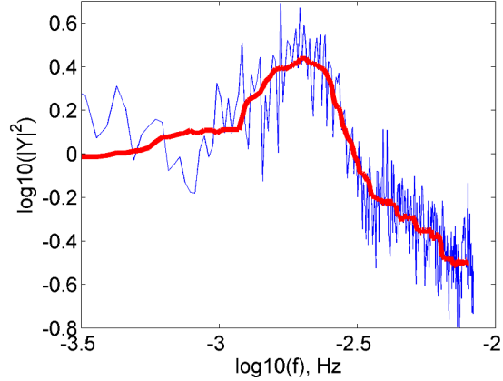
FIG. 9. Average power spectrum for 12 isolated fractures in the experiment B (blue curve) and filtered signal (red curve). The characteristic peak frequency is f_c = 2 \times 10^{-3} Hz.
