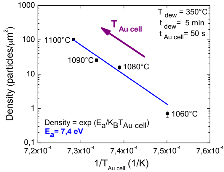
Figure 2.30 – Au-droplet surface density as a function of the inverse of the Au cell temperature. For all samples t_{Au} = 50 s, t_{dew} = 5 min, and T_{dew} = 350^\circ\text{C} .
