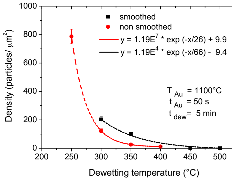
Figure 2.31 – Au-droplet surface density as a function of the dewetting temperature. For all samples: t_{dew} = 5 min, t_{Au} = 50 s and T_{Au} = 1100^\circ\text{C} . In black squares samples where the ZnTe layer was smoothed and in red circle samples where the buffer was not smoothed. The lines are exponential fits of the data.
