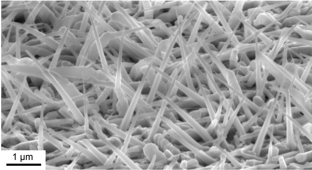
Figure 4.1 – SEM image of sample A: ZnTe coned-shaped NW grown under Te rich flux ratio conditions with a ZnMgTe shell. The image is taken with a 65^\circ angle.
