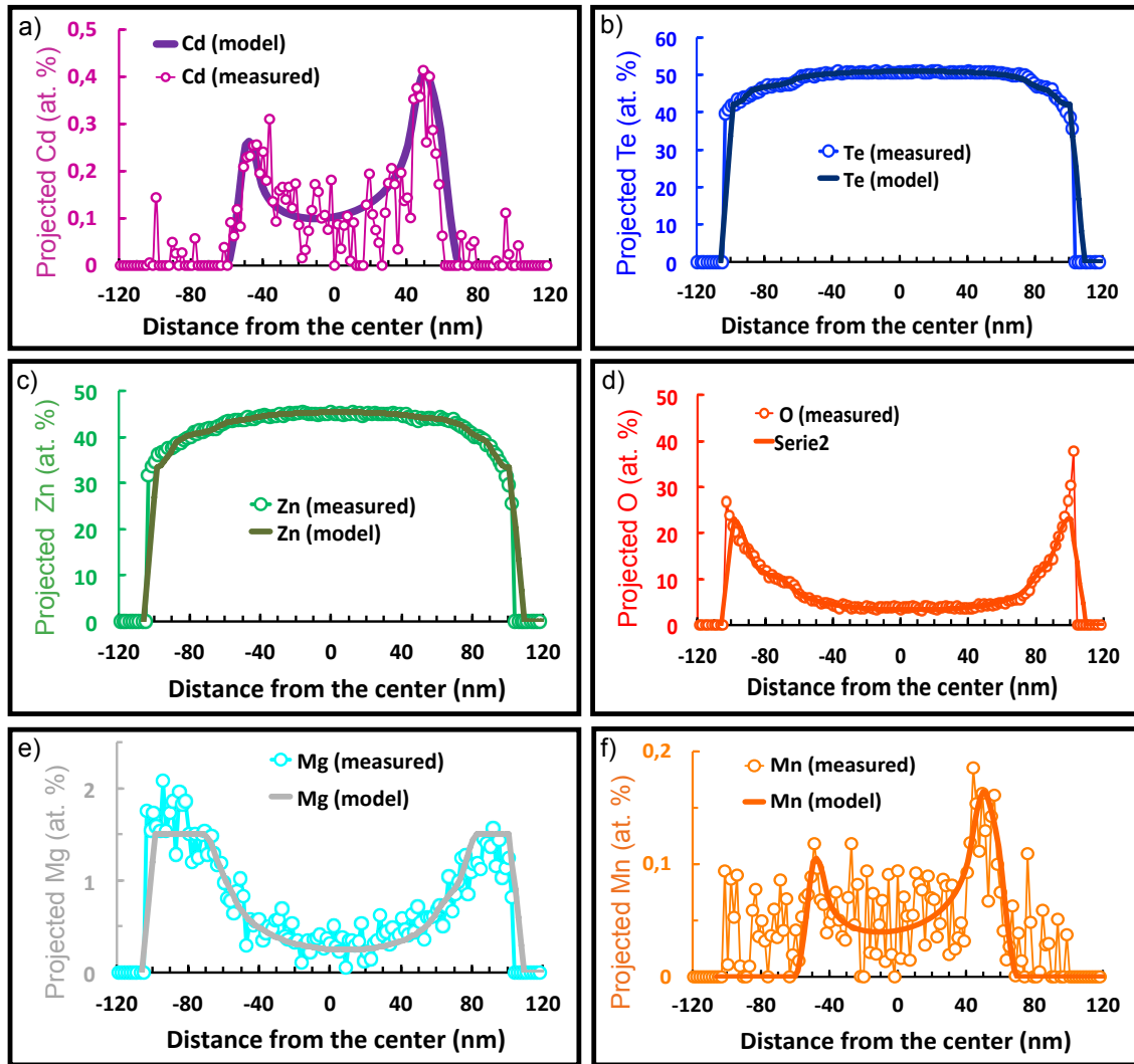
Figure 4.26 – Cd, Te, Zn, O, Mg and Mn compositions (at.%) averaged over the NW thickness obtained from the EDX map shown in Fig. 4.27 (NW from sample C). The EDX data is plotted with empty circles and the fit with continuous lines. The color code is: Cd in pink, Zn in green, Te in blue, O in red, Mn in orange and Mg in aquamarine and gray.
