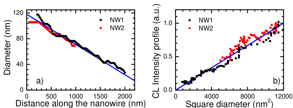
FIG. 5. (a) NW diameter as a function of the position along the NW axis for the two NWs shown in Figs. 3 and 4. (b) CL intensity (integrated over a 12 nm \times 120 nm window) as a function of the square of the NW diameter.
