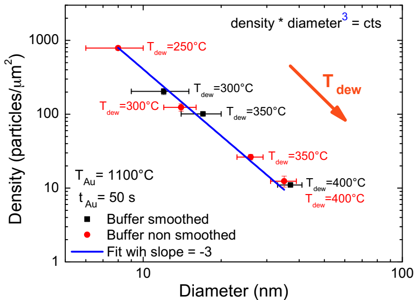
Figure 2.16 – Au-particles surface density (in logarithmic scale) as a function of the Au-particles average diameter for samples with different dewetting temperatures: T_{dew} = [250^\circ\text{C}–400^\circ\text{C}] . For all samples: t_{dew} = 5 min, T_{Au} = 1100^\circ\text{C} and t_{Au} = 50 s. In black: samples where the ZnTe buffer layer was smoothed at 420°C prior to the Au deposition at RT. In red: samples where the ZnTe buffer layer was not smoothed. The blue line is a fit of the data with a constant slope of -3. The data are obtained from SEM images of the surface.
