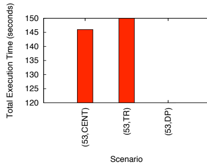
Figure 8.12: Performance of responding 10 requests per calling unit in Utopar System in different scenarios for 7 \times 7 calling units and 4 cars.
