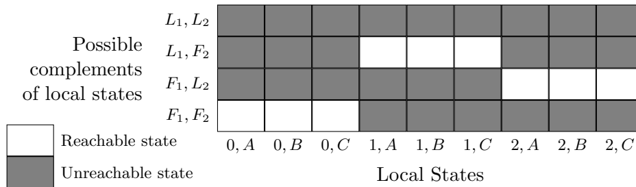
Figure 3.2: Global states of the example from Figure 2.2, decomposed by observing Jukebox and Reader processes.
