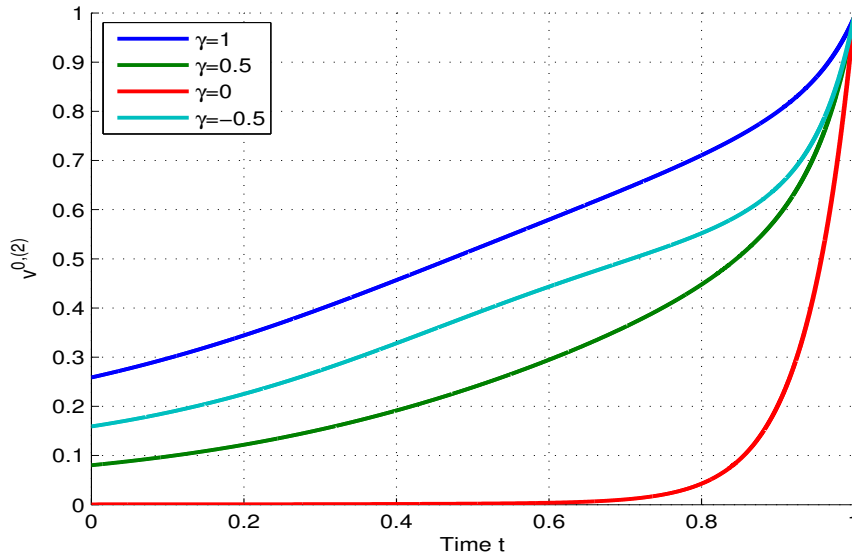
FIGURE 3.1 – v_t^0 as a function of time t \in [0, T] with T = 1 and \lambda = 0.01 for various values of \gamma .
