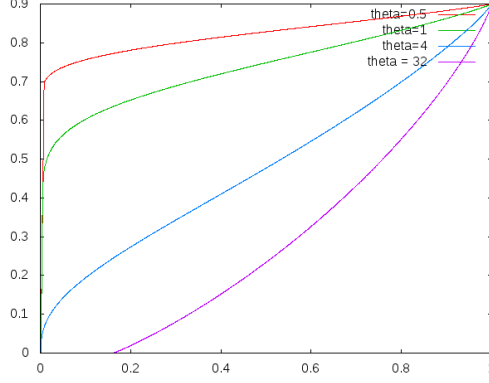
FIGURE 6.3 – Minimal weath function for constrained portfolio.
