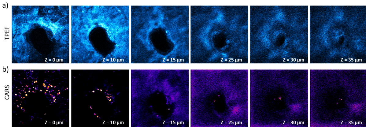
Figure 3.17: IsCC crystals distribution in sweat pore in depth (X-Y plane), image size = 100\mu\text{m} \times 100\mu\text{m} . (a) TPEF images show the morphology of sweat pore (the acrosyringium segment) up to a depth of 35\mu\text{m} . (b) CARS resonance images shows the distribution of isCC crystals at the same depth.
