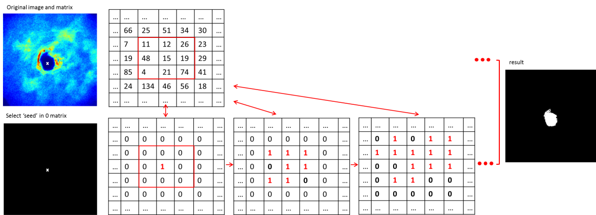
Figure 3.6: An example of “region growing method”. “Seed” point is selected manually in the original image and the neighboring pixels are in a window of 3 \times 3 pixels, the corresponding position of “seed” in 0 matrix becomes “1”; when neighboring pixels in original image agree with the conditions (see text), the corresponding position in 0 matrix becomes “1” and it becomes the new “seed”, otherwise it keeps “0”; the “1” region keeps growing until there is no neighboring pixels fulfilling the conditions.
