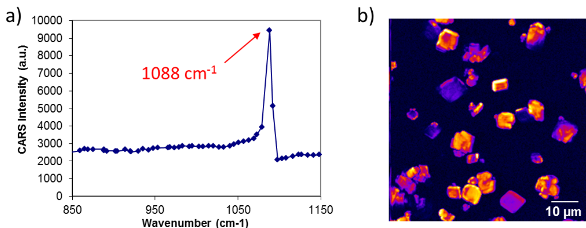
Figure 3.16: CARS spectrum and CARS on resonance image of CaCO_3 crystal (reacted from CaCl_2 and NaHCO_3 solutions). (a) CARS spectrum of CaCO_3 , the strongest vibrational signature is found at 1088\text{ cm}^{-1} in CARS signal with good signal-to-noise ratio. (b) CARS image is taken at the resonance ( = 1088\text{ cm}^{-1} ), the CaCO_3 crystals are clearly visible.
