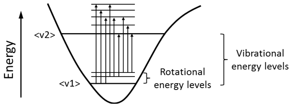
Figure 1.6: Infrared absorption.
