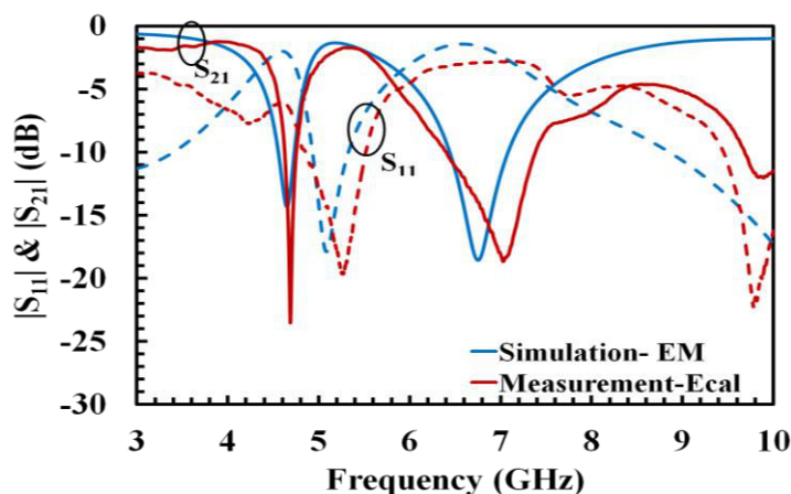
Fig. 4.54 : Simulated and measured DBR filter response on LCP Vectra E820i.
