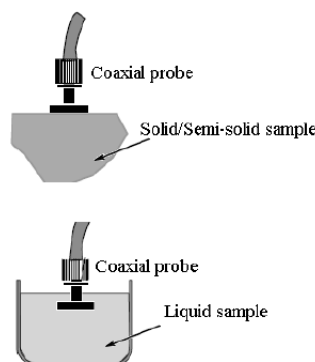
Fig. 3.4 : Coaxial probe method of characterization [19][12].
