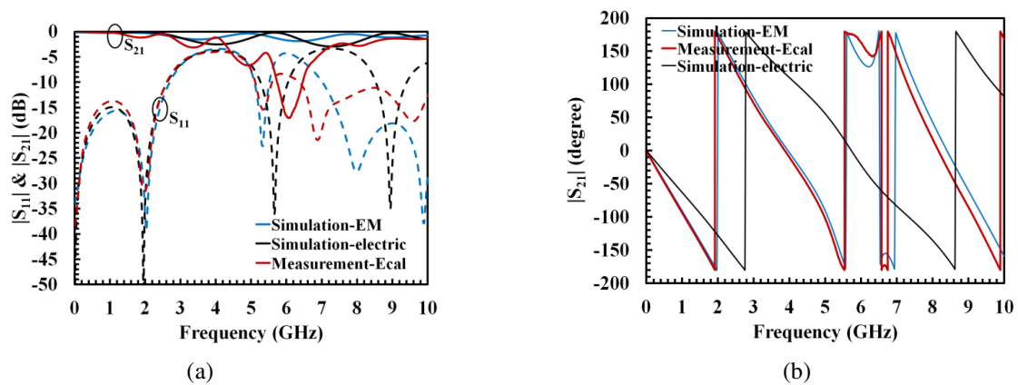
Fig. 4.18 : S parameters of MID microstrip line of length 1 cm on LCP Vectra E820i in the P_1 - P_2 planes, (a) magnitude in dB and (b) S_{21} phase in degree.
