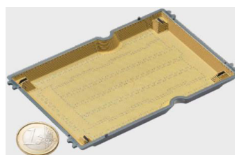
Fig. 2.22 : MID safety cap for electronic payment systems.
