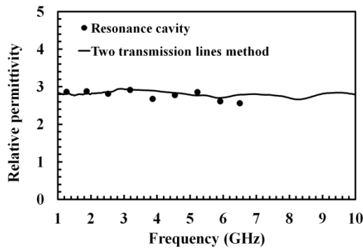
Fig. 5.6: Measured dielectric permittivity of ABS PC obtained from resonance cavity method and two transmission lines method.
