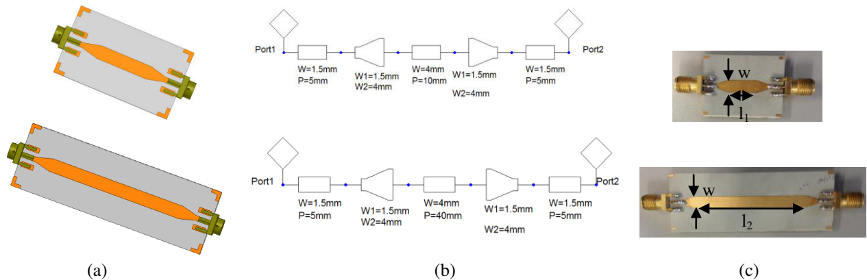
Fig. 6.2: Laser ablation transmission lines of two different lengths on LCP E130i (a) EM simulation structures, (b) electric simulation structures, and (c) fabricated photos of the lines.
