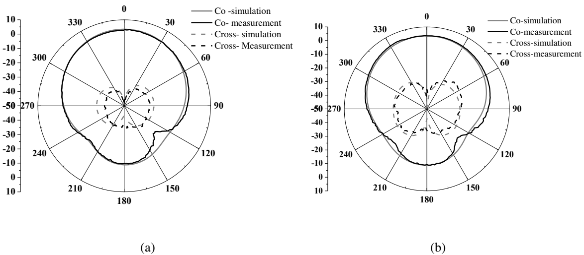
Fig. 5.18 : Measured and simulated radiation pattern of MID microstrip patch antenna on ABS PC (a) the H plane and (b) the E plane.
