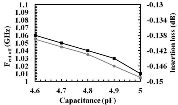
Fig. 4.48 : variation in CPW HLPF cut off frequency with respect to capacitance variation.
