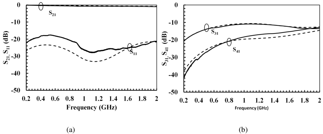
Fig. 6.22 : Simulated and measured S parameters of three section directional coupler on high K thermoplastic material (a) return loss and insertion loss and (b) isolation and coupling.
