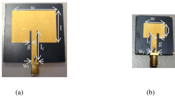
Fig. 4.58 : LDS MID antenna structures on LCP Vectra E820i: (a) at 2.63 GHz and (b) at 5.8 GHz.
