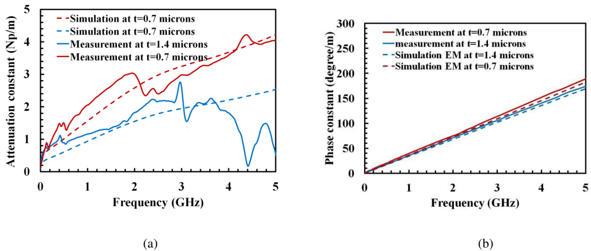
Fig. 5.43 : Propagation constant of inkjet printed MID microstrip transmission line on planarized LCP E130i with metal thickness of 0.7 \mu m and 1.4 \mu m, (a) attenuation constant and (b) phase constant.
