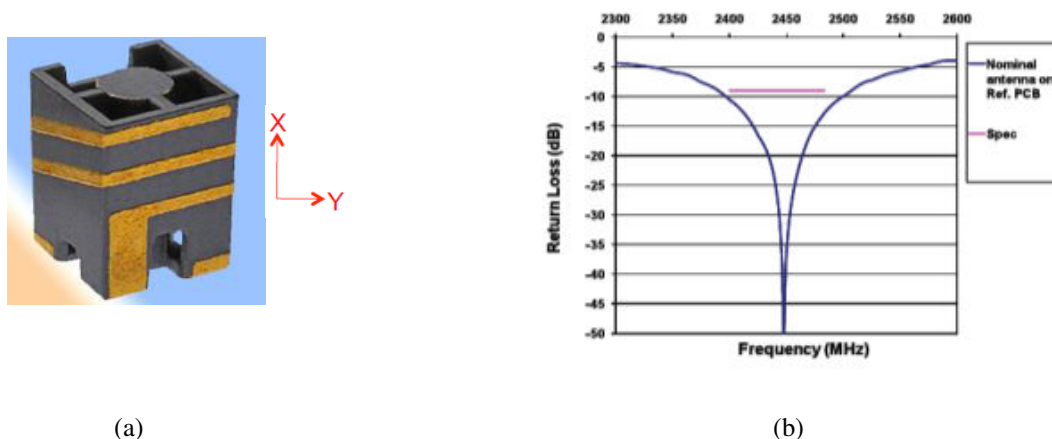
Fig. 2.12 : Smallest on-ground MID antenna, (a) fabricated antenna prototype, and (b) its reflection coefficient.
