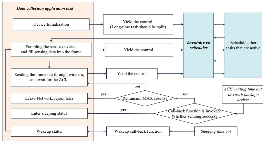
Figure 5.1: Flowchart of WSN environmental data collection application.
