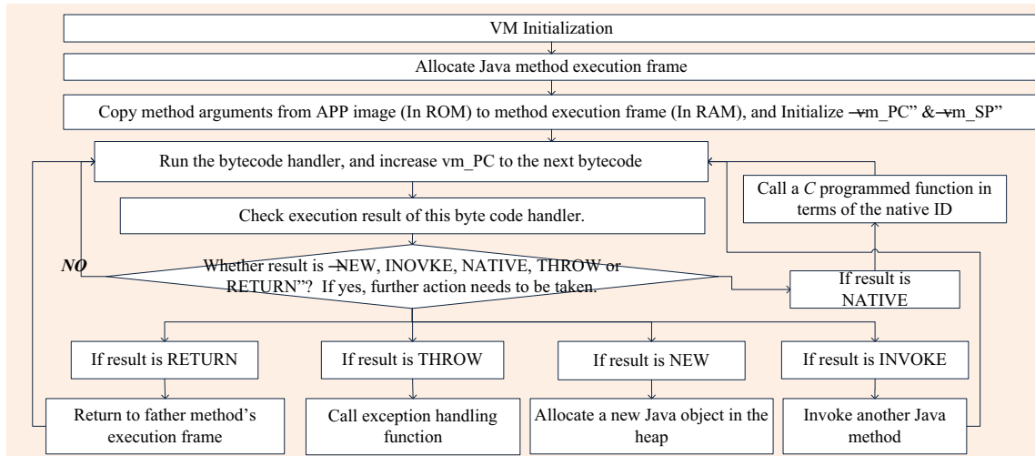
Figure 4.6: Java bytecode interpretation process in simpleRTJ.
