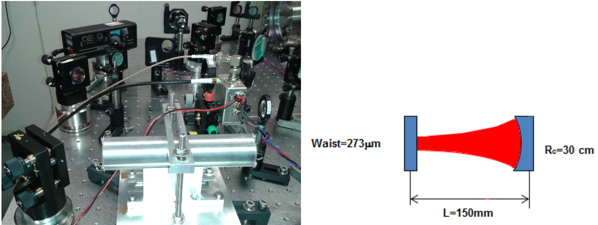
Figure 7.11: Real picture and scheme of the linear cavity used for the optimization and ‘cleaning’ of the higher order HG modes.
