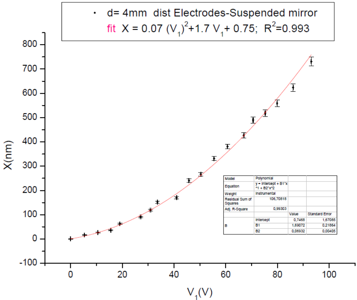
Figure 6.12: Graphic of the fit on the best collected sample. The data show a law X \propto V_1^2 as expected. The maximal displacement reached is \sim 800\text{nm} for an applied rms voltage on the capacitor of V_1 = 100\text{V} while the capacitor is at the closer distance d = 4\text{mm} to the suspended mirror, as expected too. The mirror here is suspended with two ears and my hair as suspension wire (see fig.6.9).
