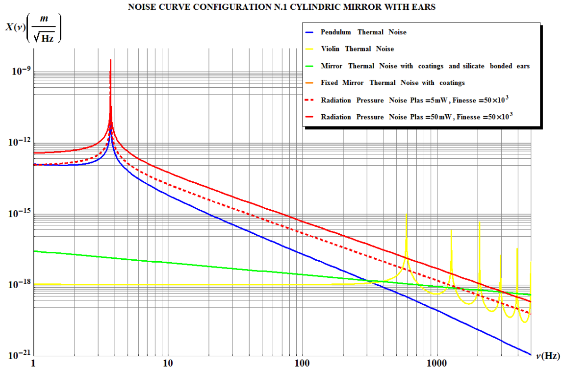
Figure 4.7: Noise Budget for the Cylindrical mirror with silicate bonded ears (configuration n.1). The Quantum Radiation Pressure Noise with laser power 5mW (red dashed curve) and 50mW (red curve) are higher than the Pendulum Thermal Noise (blue curve), the Violin Thermal Noise (yellow curve) and the Mirror Thermal Noise (green curve). The last one is much lower, but the pendulum thermal noise is not low enough compared to the radiation pressure noise in the detection band.
