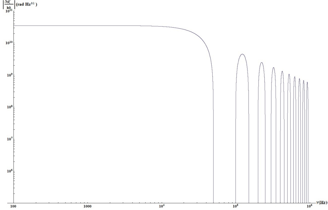
Figure 1.11: Frequency response of an interferometer with arms length L = 3\text{km} and laser wavelength \lambda_L = 1.064\mu\text{m} .
