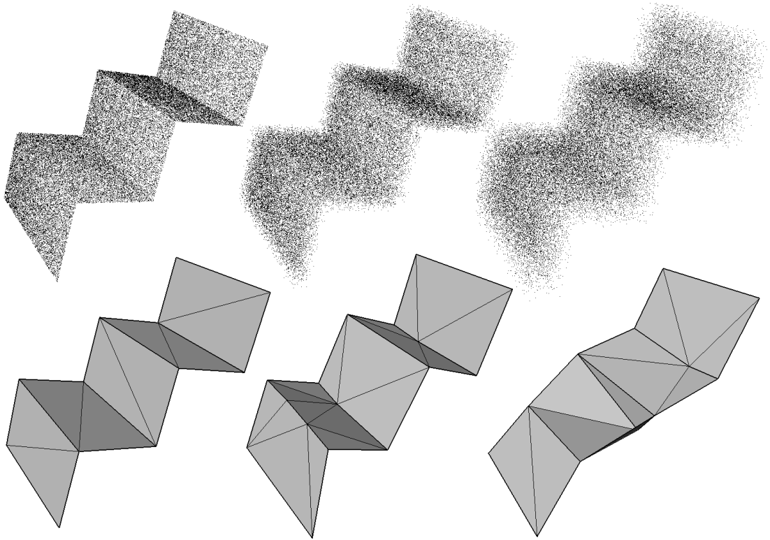
Figure 9.16: Noise robustness. Top: input point cloud with increasing level of noise. Bottom: output mesh using a noise threshold \epsilon_N of respectively 0.005, 0.050 and 0.200.
