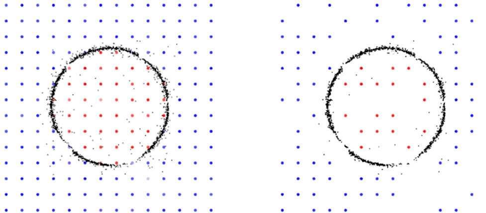
Figure 5.13: Confidence filtering. Left: result of the sign guess. Right: sign guesses with a confidence \geq c_{min} = 0.75 .
