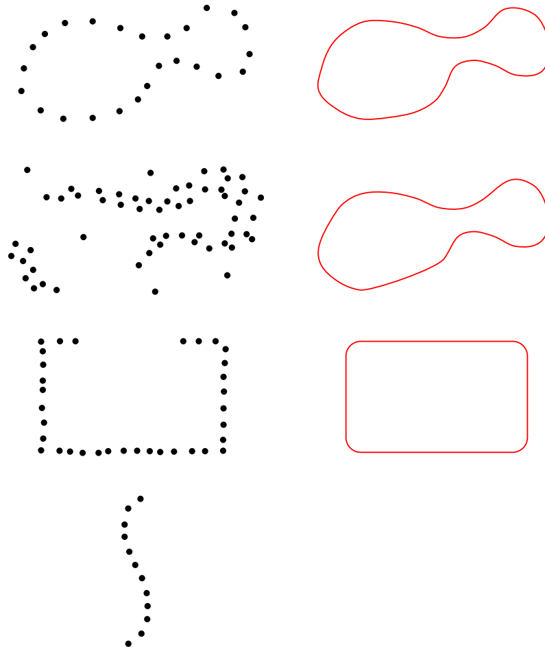
Figure 3.1: Plausible reconstructions. Left column: input point cloud. Right column: plausible smooth closed reconstruction. The last point cloud does not sample the border of a domain and cannot be reconstructed.
