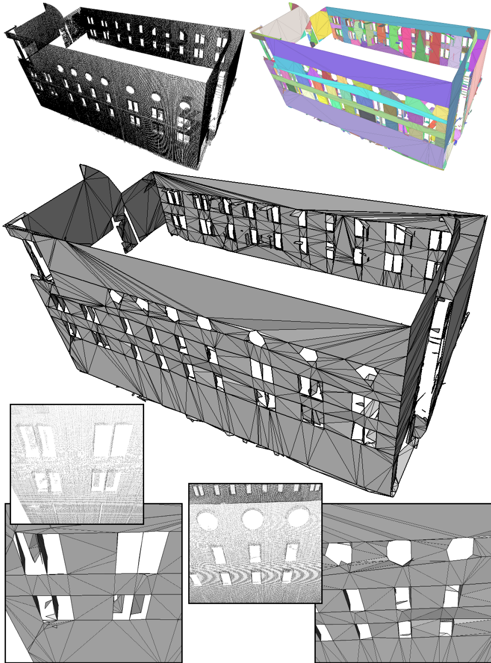
Figure 9.12: Building . Input LIDAR point cloud (top), colored primitives, output simplifical mesh, and two close-ups (bottom).
