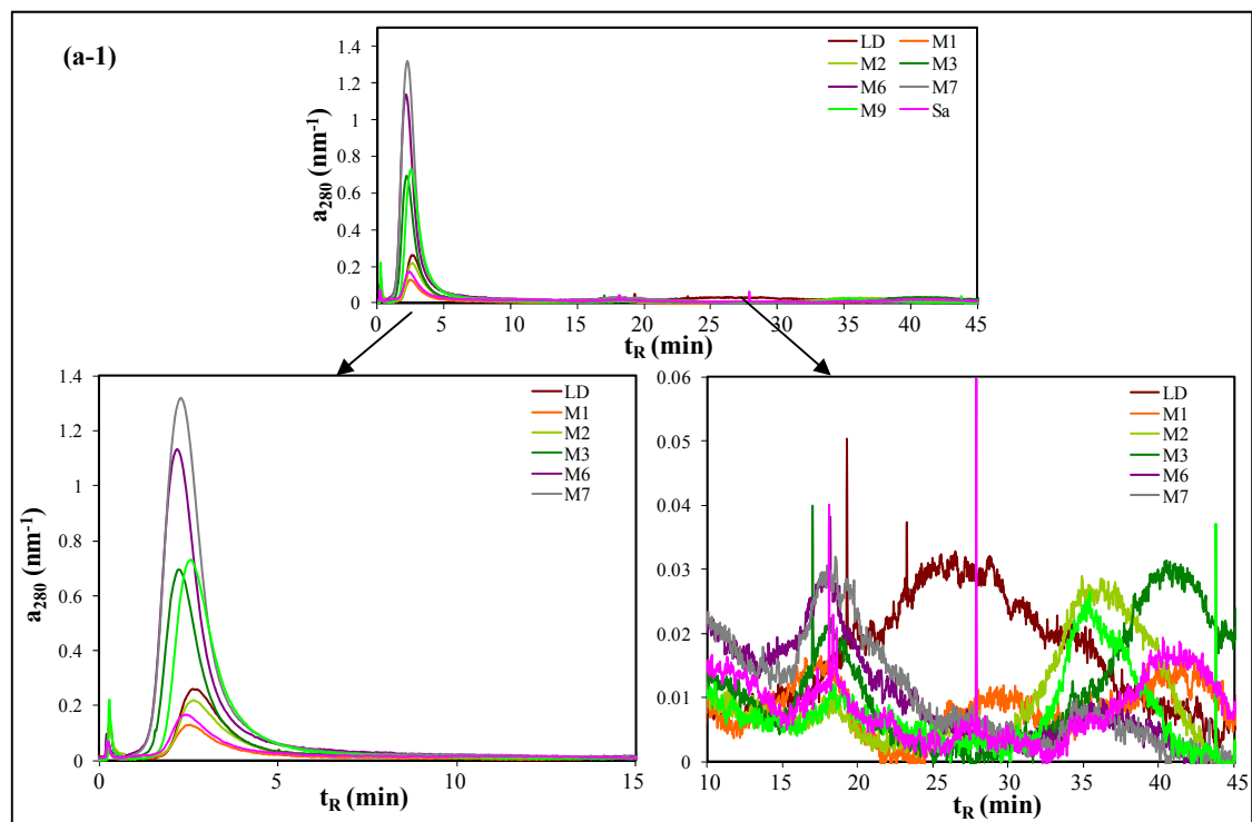
Appendix 3-b: Fractogram of samples collected in 2013 within the Seine River catchment obtained by AF4. (a-1) Marne River and (a-2) Grand Morin tributary; (b-1) Oise River and (b-2) its tributaries; (c-1) Seine River and (c-2) its tributaries
