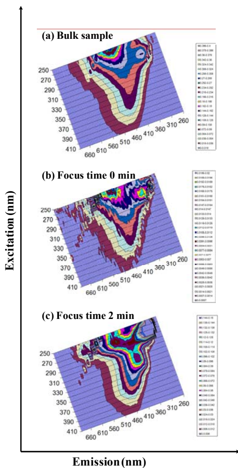
Figure 4.6 EEM spectra of (a) bulk sample Mery (S1- 2012), (b) fraction collected for t_f=0 min, (c) fraction collected for t_f=2 min
