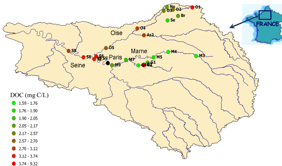
Figure 3.1 DOC concentrations for samples collected in November 2011 (Varrault et al., 2013)
