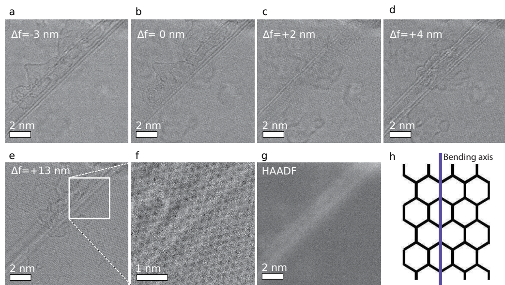
Figure 4.6: a-e. Five micrograph of two couples of parallel fringes extracted from a 34-images focal series. The two pairs of fringes are focused at different focal depths. f Magnified image showing that the fringes are aligned along an arm-chair direction of the h -BN lattice. g. Dark field image of the region showing a local increase of the projected density at the fold. h Bending axis observed at the fold.
