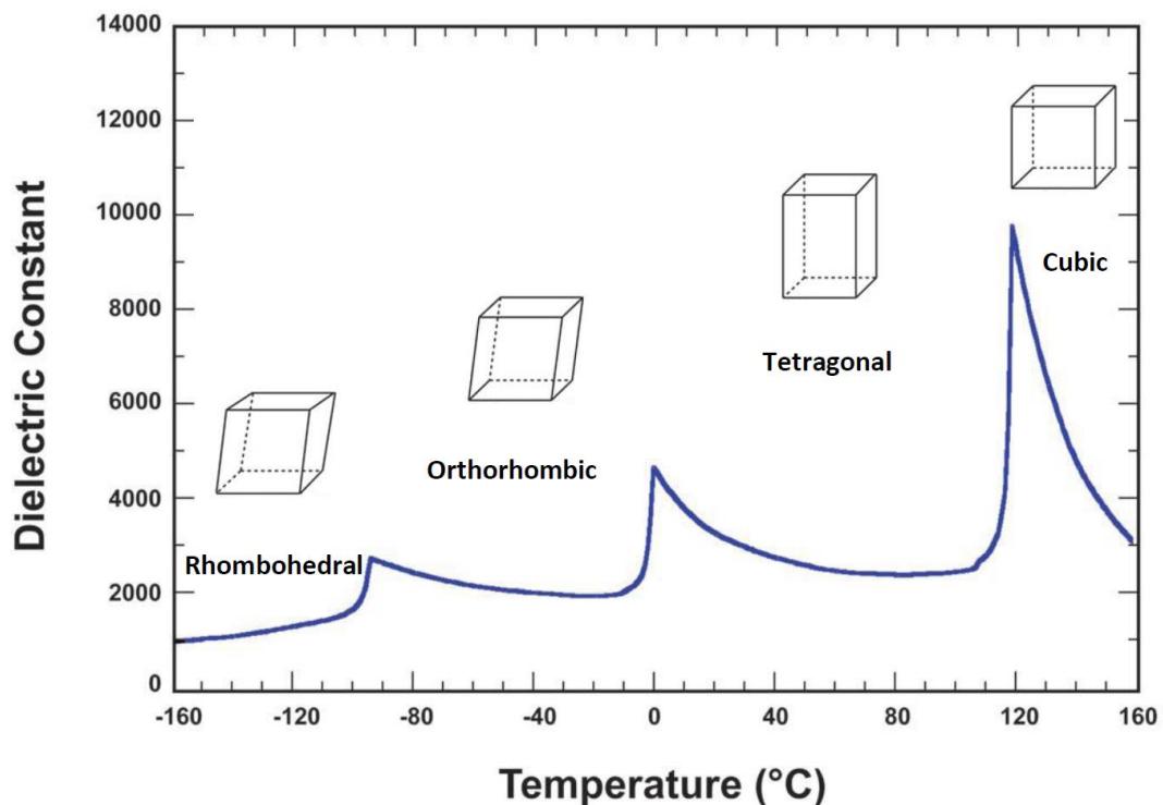
Figure I-15. Evolution of BaTiO_3 dielectric permittivity as a function of temperature [19] Copyright © 2010, IEEE.
