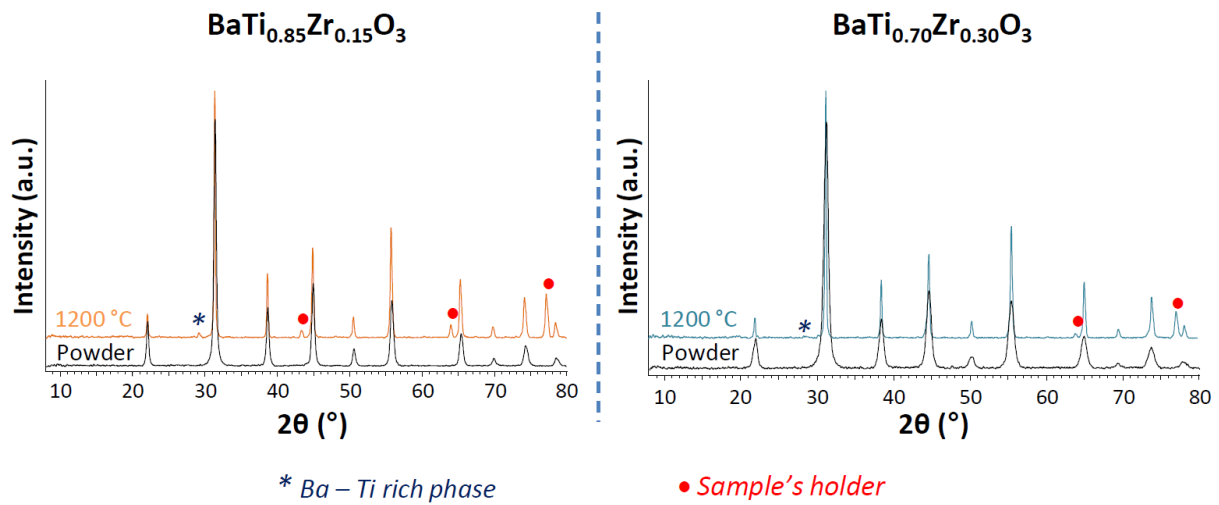
Figure IV-28. XRD patterns of \text{BaTi}_{0.85}\text{Zr}_{0.15}\text{O}_3 and \text{BaTi}_{0.7}\text{Zr}_{0.3}\text{O}_3 powders and ceramics sintered at 4 hours at 1200^\circ\text{C} .
