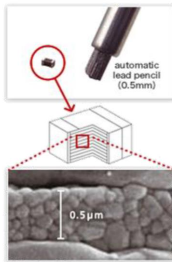
Figure I-8. Submicron layer of a MLCC.
