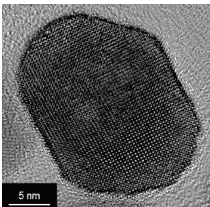
Figure 3: Nanocristal de \text{BaTiO}_3
