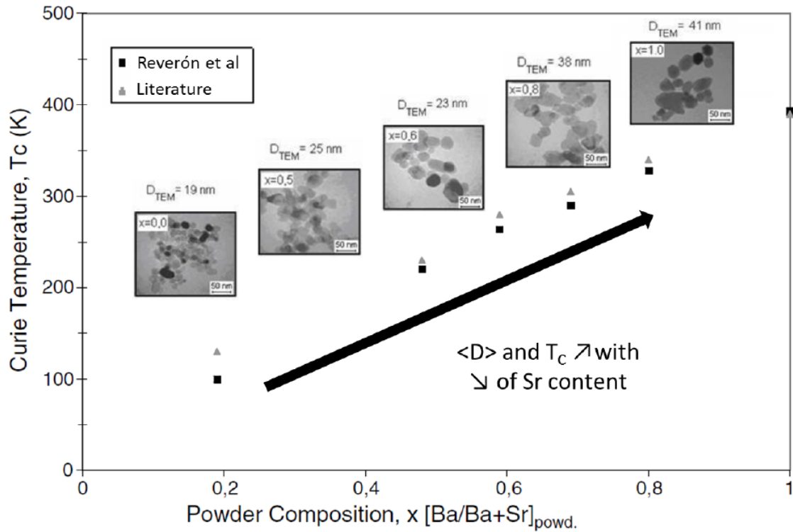
Figure I-34. Effect of barium substitution with strontium on particles size T_{Curie} evolution [189].
