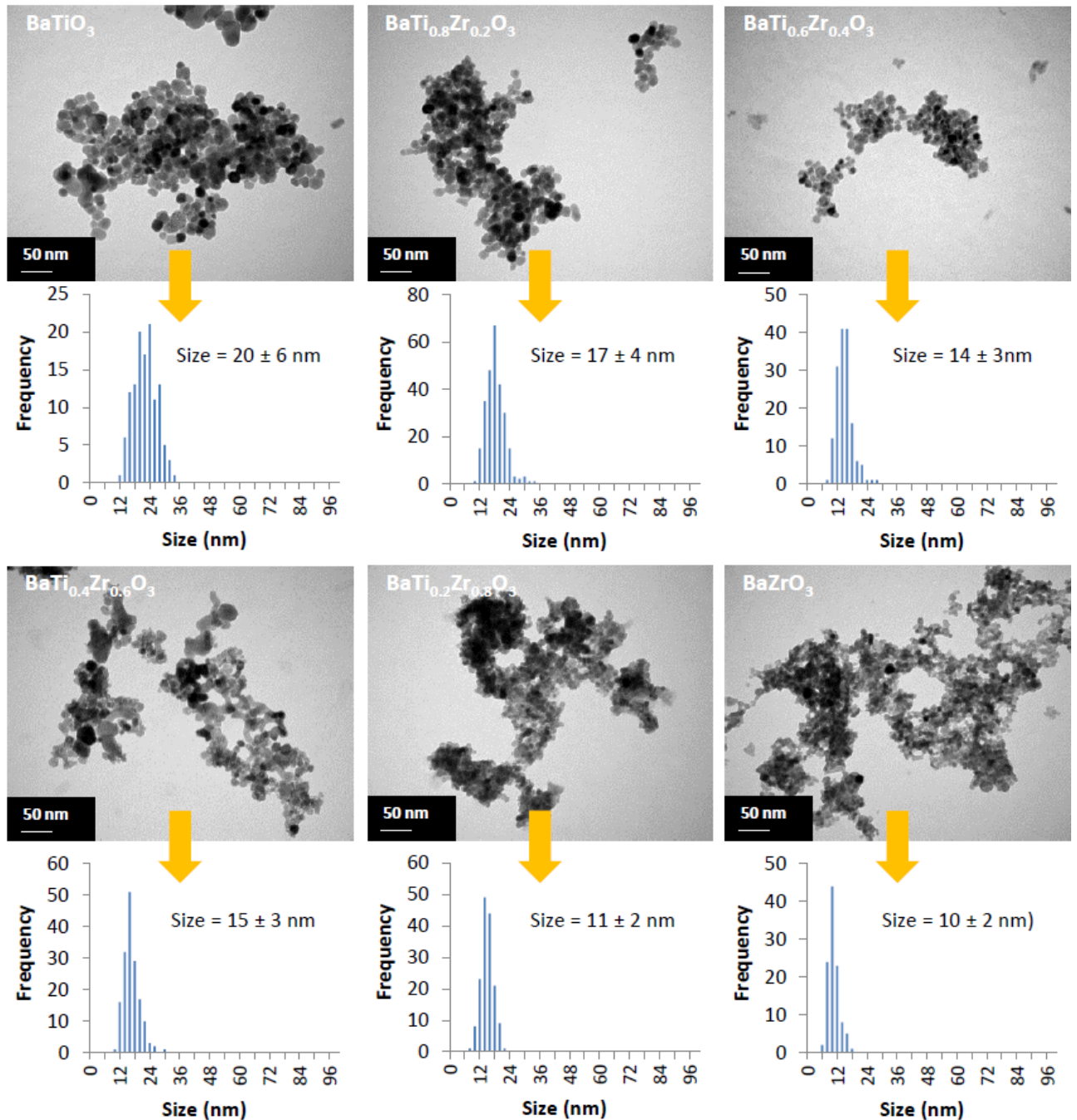
Figure III-26. TEM images of BTZ nanoparticles synthesized according to the material composition.
