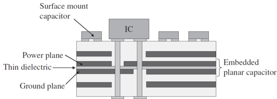
Figure I-11. Illustration of an embedded capacitor configuration [23] Copyright © 2011, Elsevier.
