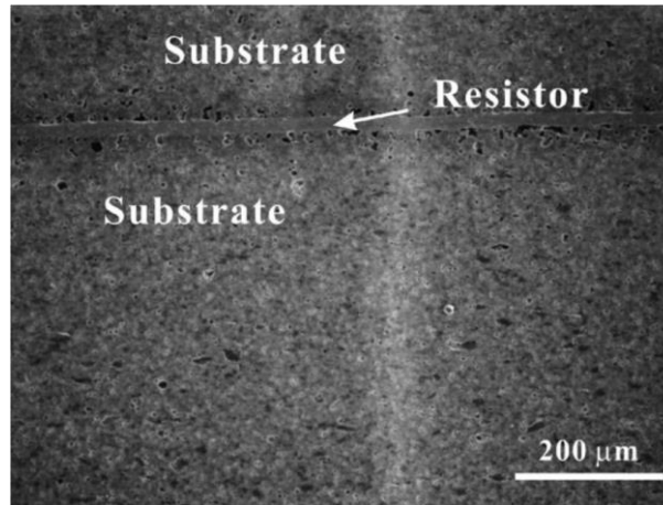
Figure I-12. Illustration of an embedded ceramic resistor made by co firing of the dielectric and substrate [24] Copyright © 2007, Elsevier.
