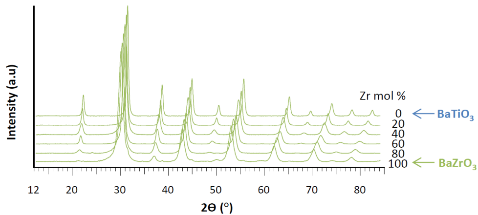
Figure III-24. XRD patterns of the BTZ solid solution exhibiting a regular shift towards smaller 2\theta angles from BaTiO_3 to BaZrO_3 .
