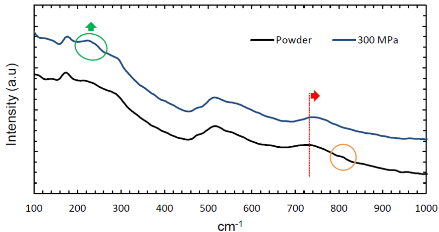
Figure IV-5. Room temperature Raman analysis of the BST powder before and after SPS processing. Very interesting information could be pulled of this analysis and compared to the literature [264]:
