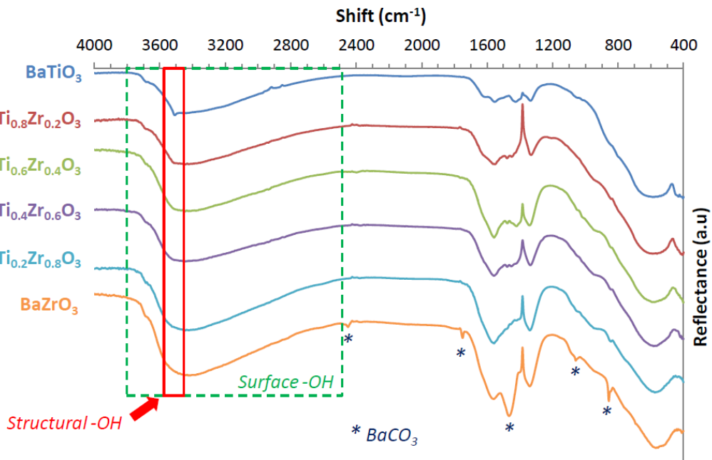
Figure III-29. FTIR of the various BTZ compositions confirming the \text{BaTiO}_3 purity preservation excepts for \text{BaZrO}_3 where a \text{BaCO}_3 contamination is observed, and exhibiting the presence of surface and structure -\text{OH} defects
