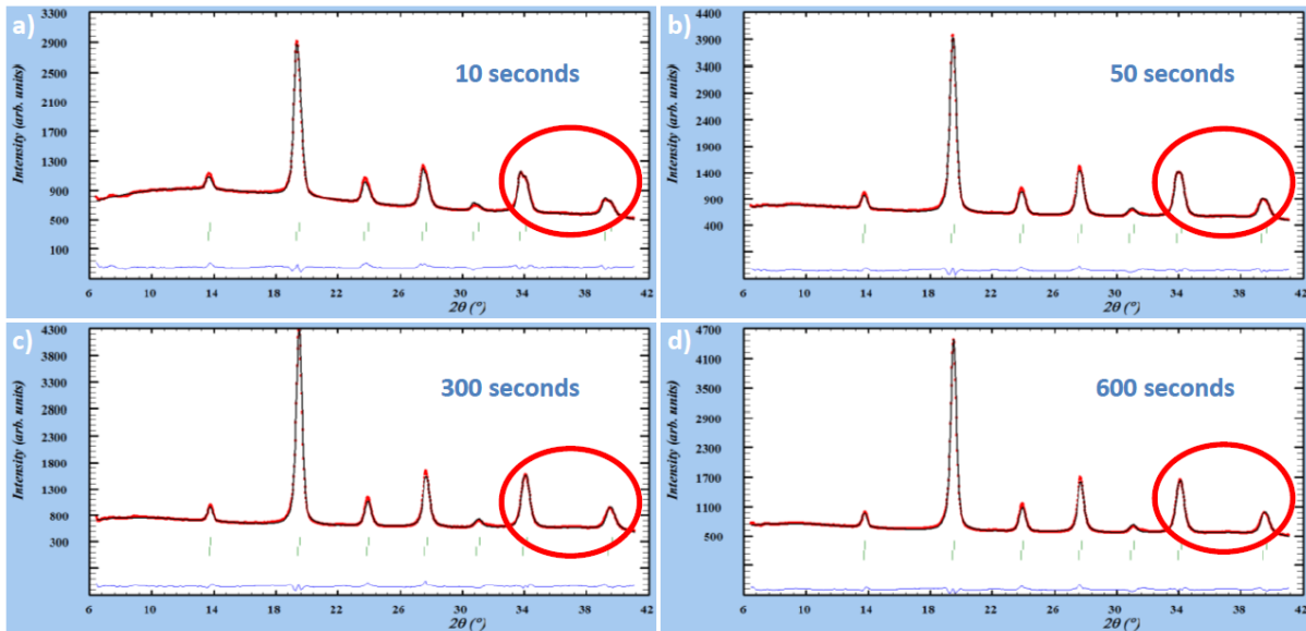
Figure III-31. In situ studies of the \text{BaTi}_{0.4}\text{Zr}_{0.6}\text{O}_3 synthesis: decrease of the powder diffraction pattern splitting with time.
