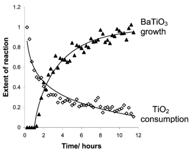
Figure I-29. In situ neutron diffraction experiment showing of the consumption of TiO 2 and growth of BaTiO 3 with time [129] Copyright © 2001, American Chemical Society.
