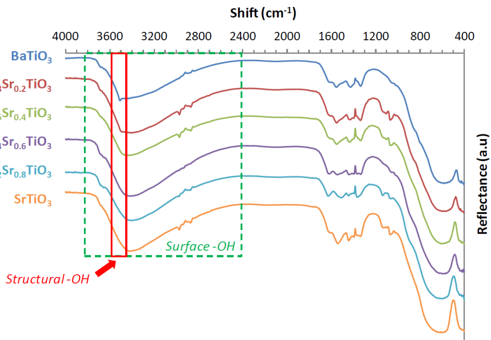
Figure III-21. FTIR spectra of the various BST compositions confirming the \text{BaTiO}_3 purity preservation and exhibiting the presence of surface and structure \text{-OH} defects
