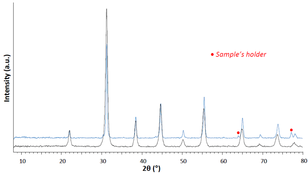
Figure IV-36. XRD pattern of the \text{BaTi}_{0.7}\text{Zr}_{0.3}\text{O}_3 powder (black) ceramic (blue) sintered with SPS (3 minutes at 1200^\circ\text{C} and 100\text{ MPa} ).
