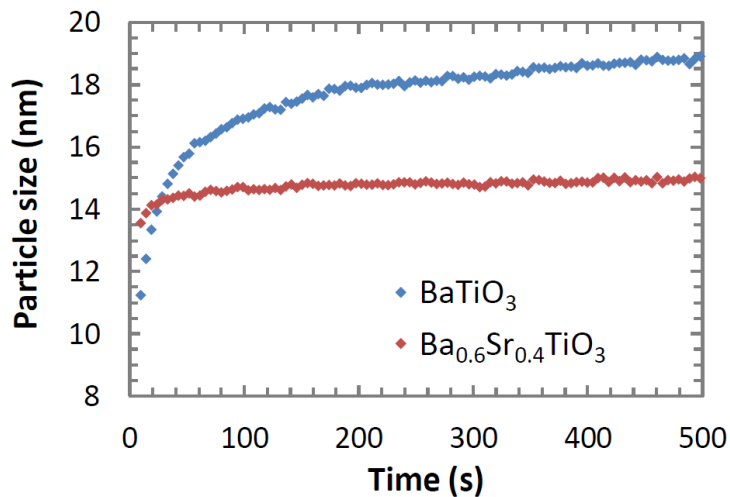
Figure III-19. In situ study of the strontium effect on particles growth at T = 400\text{ }^{\circ}\text{C} and P = 23\text{ MPa} .
