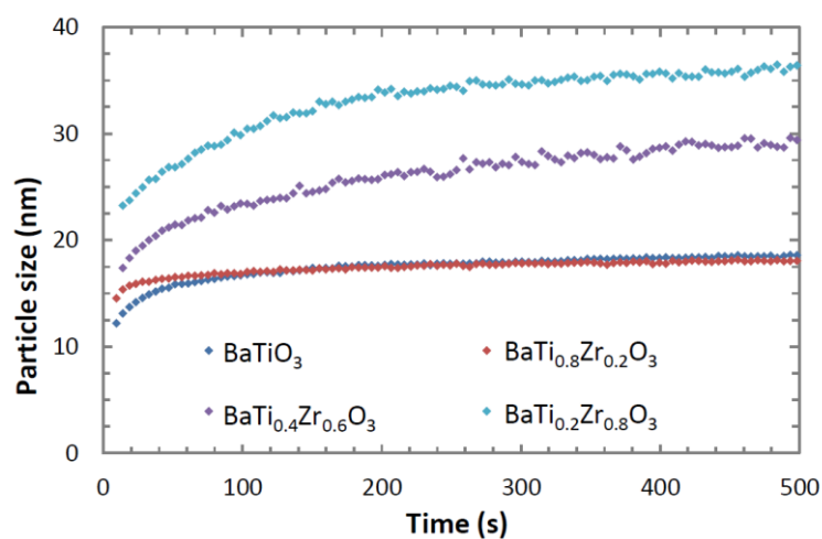
Figure III-32. In situ study of the zirconium effect on to particles growth at T = 400\text{ }^\circ\text{C} and P = 23\text{ MPa} .
