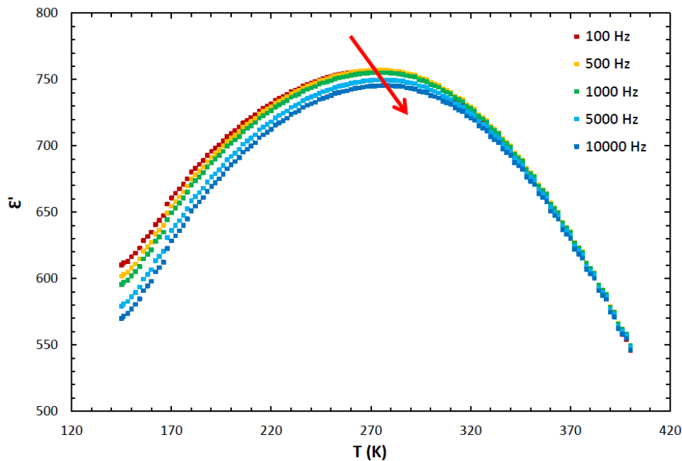
Figure IV-37. Dielectric measurement of the \text{BaTi}_{0.7}\text{Zr}_{0.3}\text{O}_3 ceramic sintered with SPS (3 minutes at 1200^\circ\text{C} and 100\text{ MPa} ).
