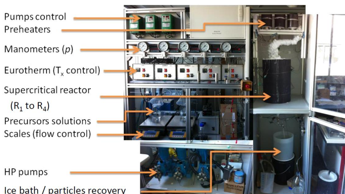
Figure II-2. Photography of the continuous flow experimental setup used for the synthesis of nanoparticles in supercritical fluids.
