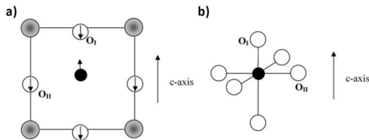
Figure I-17. Apparition of spontaneous polarization with cell distortion in P4mm space group : a) displacement of the \text{Ti}^{4+} cation and \text{O}^{2-} anions in opposite directions and b) non centrosymmetric octahedron [18].
