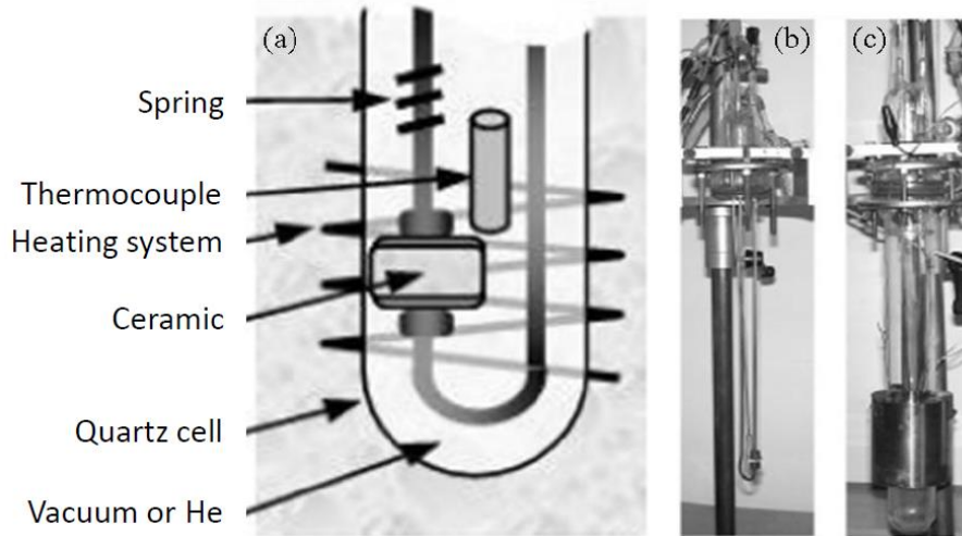
Figure II-8. a) sketch of the dielectric measurement cell, b) image of the open cell and c) image of the closed cell.
