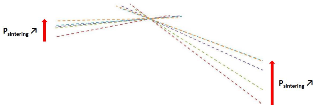
Figure IV-20. Superimposition of the fits of Figure IV-18 for determining the position of the T_{Curie} . Reporting the T_{Curie} as a function of the applied pressure during sintering (Figure IV-21) evidences an increase of the transition temperature from \approx 180 K up to \approx 207 K when the pressure increases respectively from 300 to 400 MPa and then remains stable in a second regime from 400 to 600 MPa.
