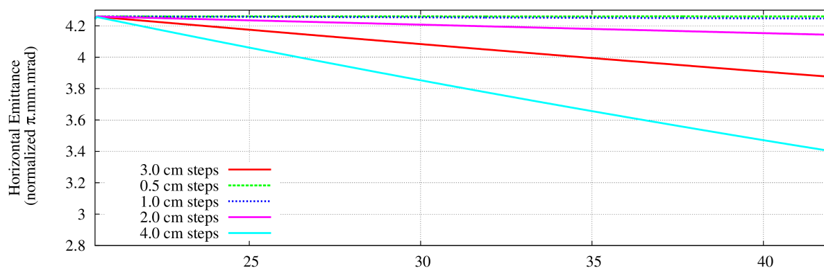
Figure 4.16 Evolution of the single particle horizontal normalized emittance for a 80,000 turns tracking using the AGS bare model.
