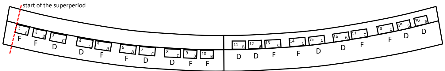
Figure 2.4 Synoptic drawing of one AGS superperiod with the opened side of each magnet facing the centerline. Magnet number, type and function is also labeled. The start of the superperiod is by convention at the magnetic edge of the first main magnet.
