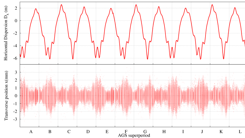
Figure 4.18 Horizontal dispersion and transverse beam position during tracking, at G\gamma = 15.7 .
