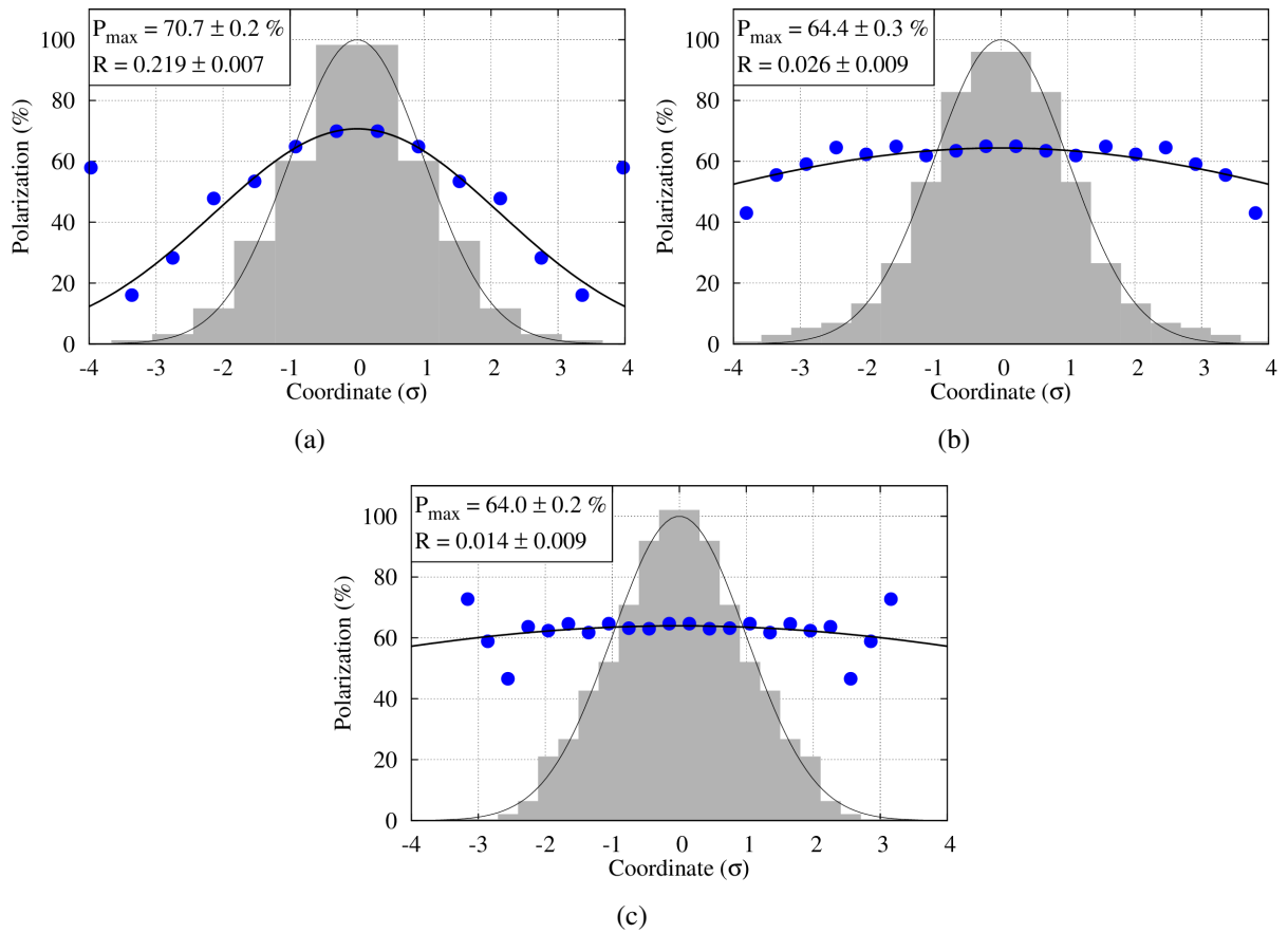
Figure 4.10 Polarization profiles at G\gamma = 45.5 from beam multiturn Zgoubi tracking in the AGS in the horizontal (a), vertical (b) and longitudinal (c) planes.
