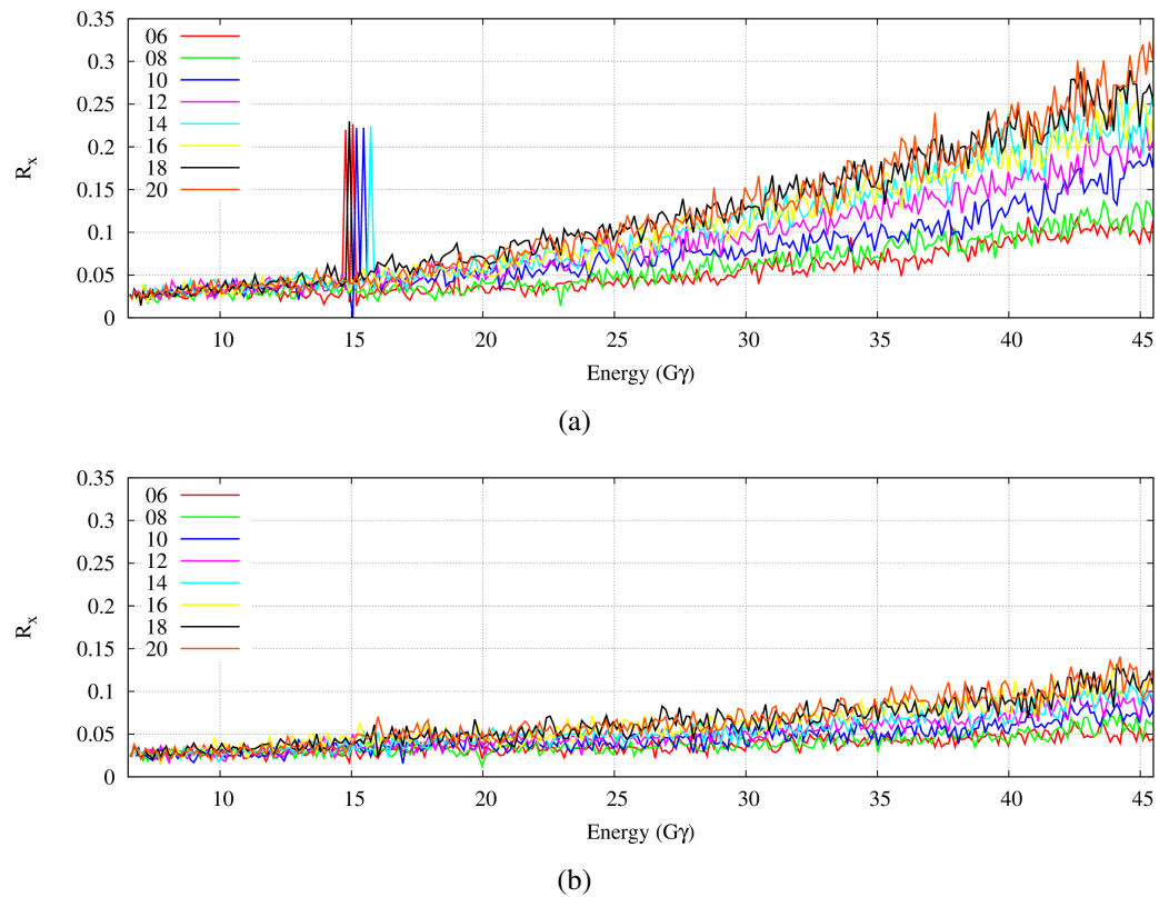
Figure 4.20 Simulated horizontal polarization profile as a function of the energy for different initial beam horizontal emittances (in 95\% \pi mm.mrad normalized and at G\gamma = 6.5 ) without (a) and with tune jumps (b).
