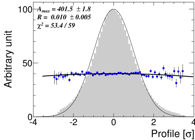
Figure 5.14 Measured vertical polarization profile at G\gamma = 7.5 with vertical tune jumps.
