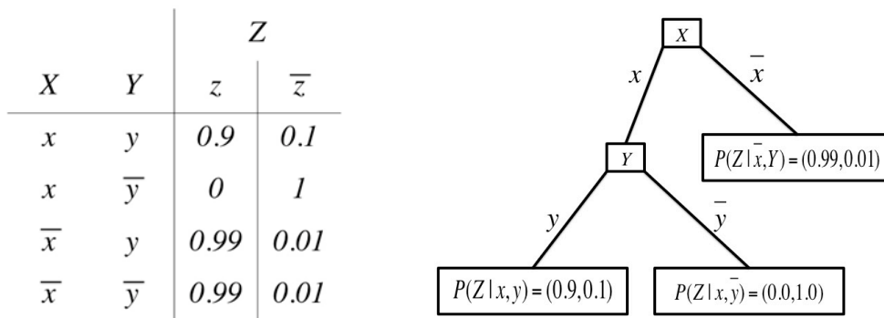
Figure 31. CPT and tree exposing local structure within the conditional probability distribution.
