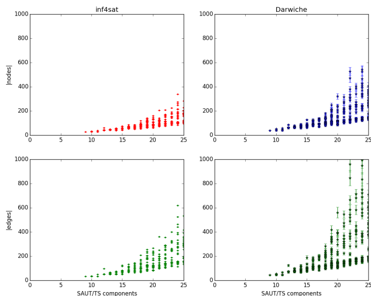
Figure 54. Comparison of compilation size results with variance.
