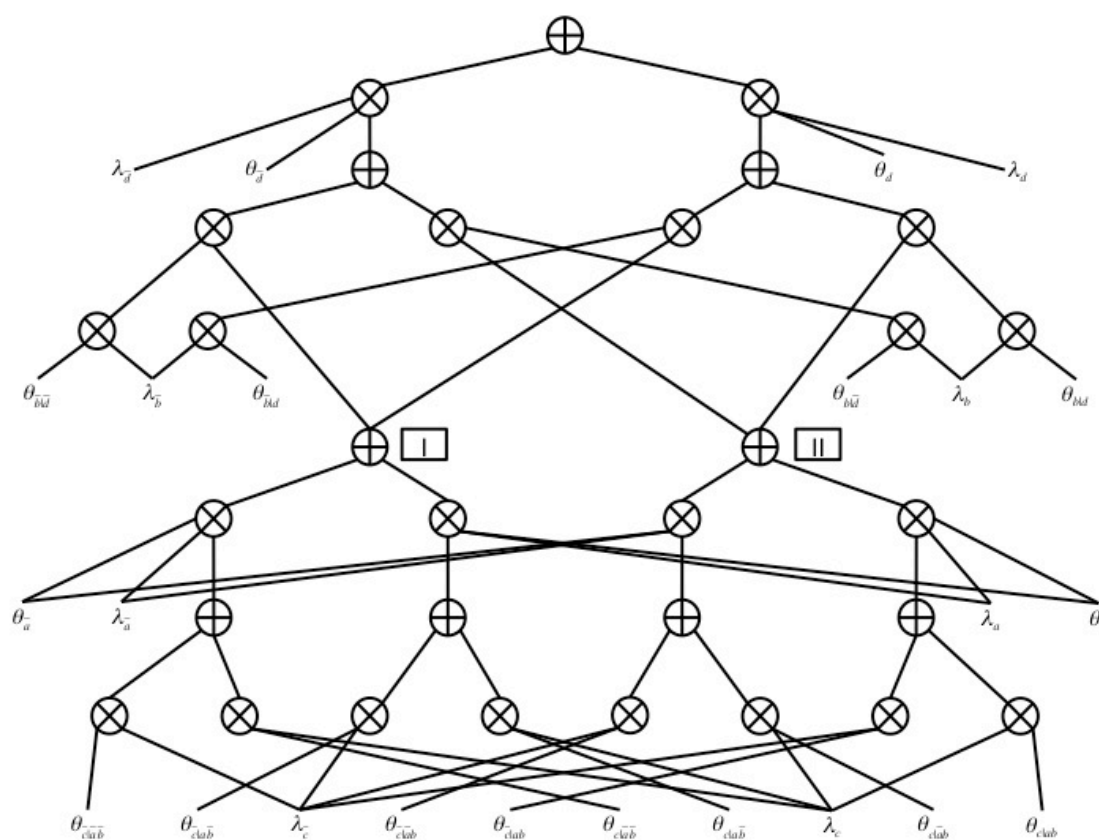
Figure 36: Example of an Arithmetic Circuit.
