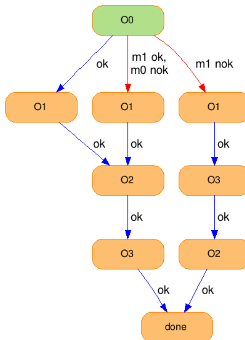
Figure 51. Sequence diagram of three path of test sample execution according to the returned verdicts.
