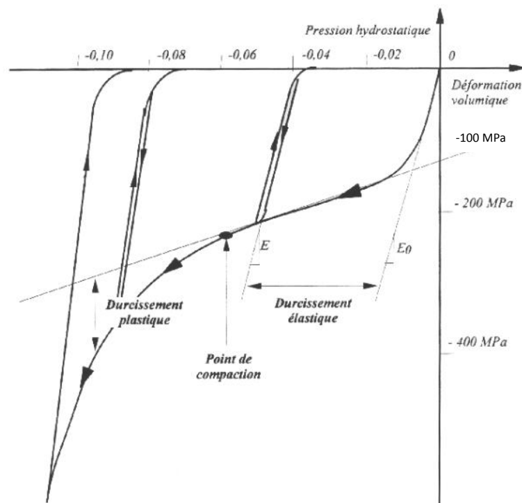
Figure 12 - Comportement compactant du béton (Burlion, 1998).
