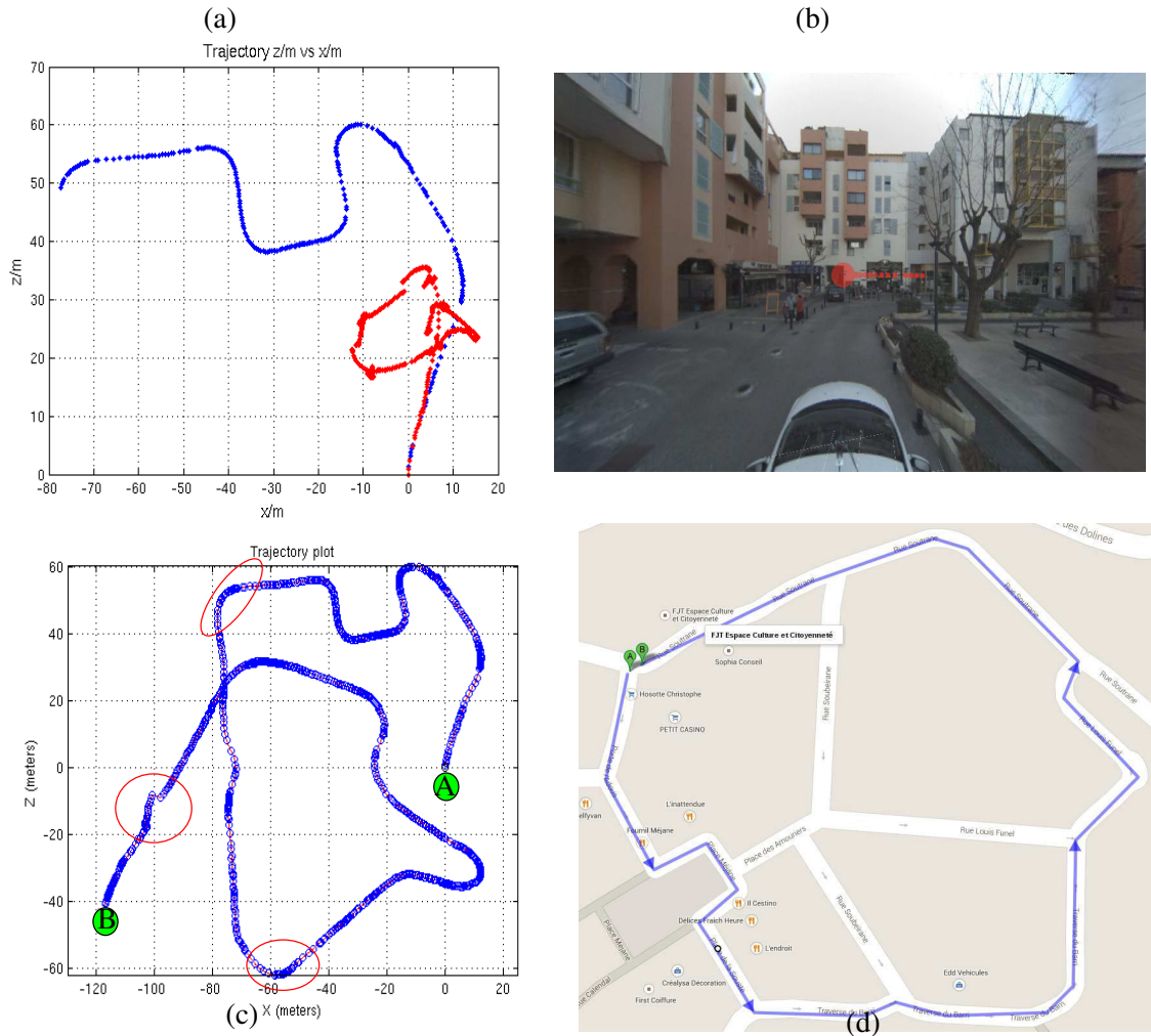
Figure 4.24: Degenerate conditions and VO failures on full trajectory reconstruction
