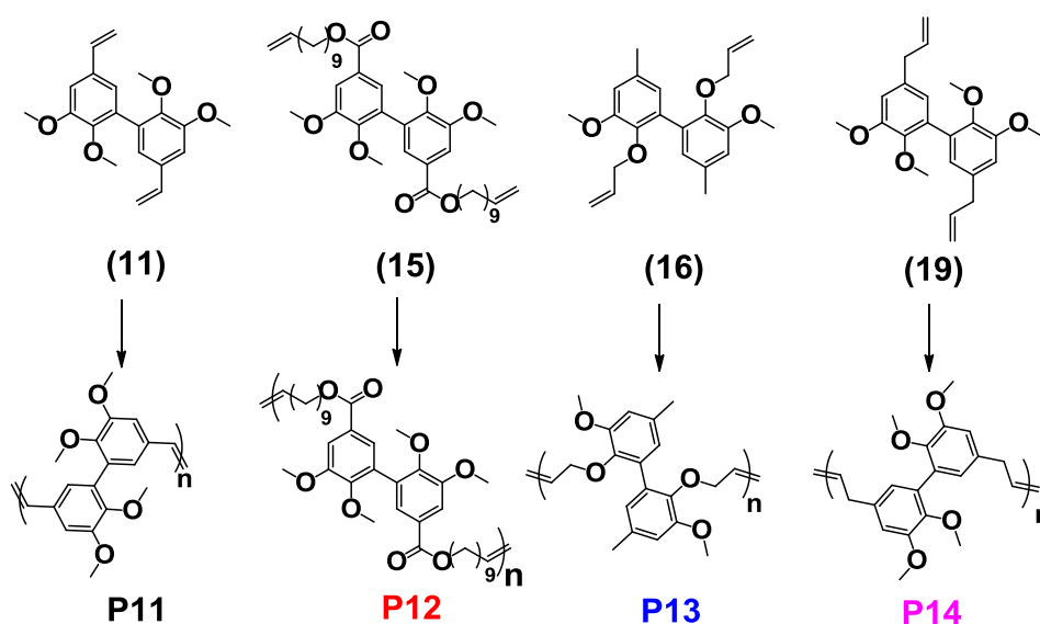
Scheme 5: Structures of the polymers P11 , P12 , P13 and P14 synthesized by ADMET polymerization from divanillic divinyl ( 11 ), bis-unsaturated diester ( 15 ), allylated 4-methyl-2-methoxy dimer ( 16 ), methylated and dieugenol ( 19 ).
