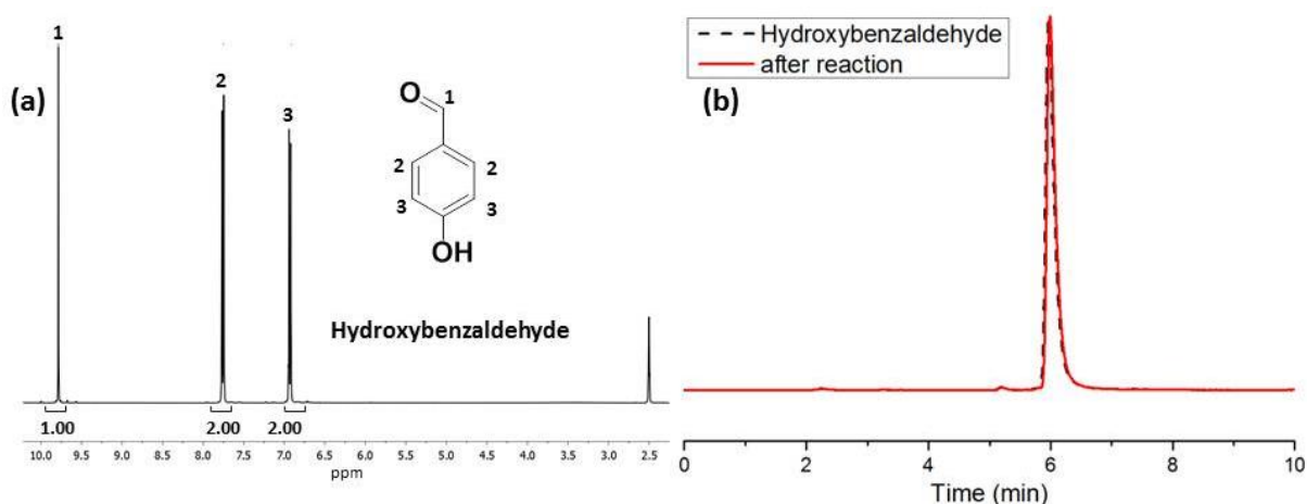
Figure 13: ^1\text{H} NMR spectrum in DMSO at room temperature (a), HPLC profile using a C18 grafted silica column and acetonitrile as eluent (b) of product formed by coupling hydroxybenzaldehyde catalyzed by laccase.
