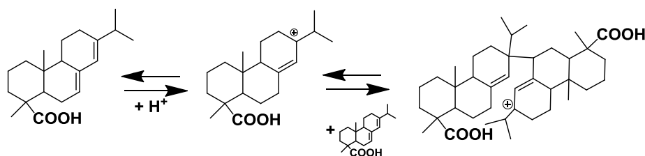
Scheme 1: Proposed mechanism for abietic acid dimerization. 3
