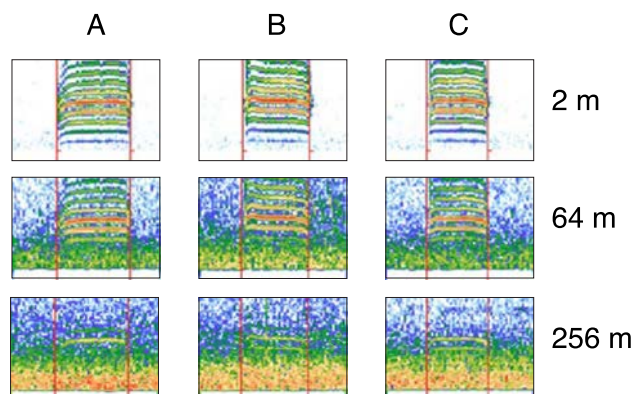
Fig. 8: Coordinates for the beginning and ending of 3 calls (A, B and C) at 3 propagation distances. Note that the color scale for the spectrograms is different for each distance.
