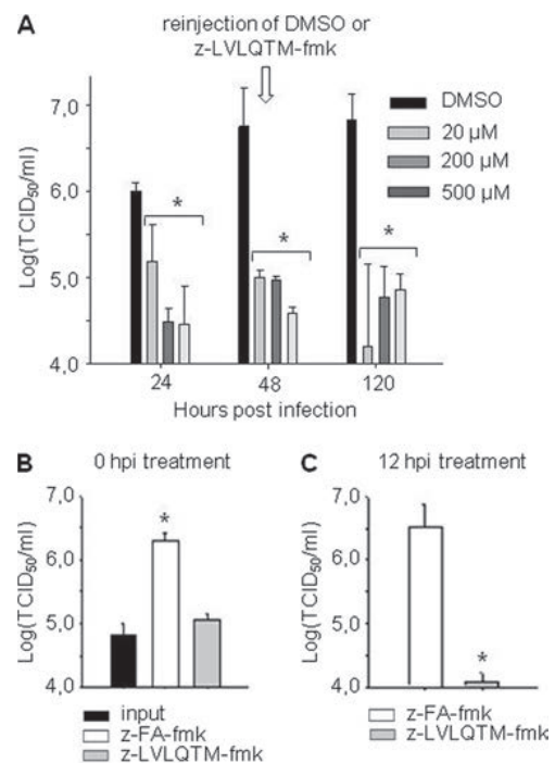
FIG 8 z-LVLQTM-fmk specifically inhibits HRV replication in vivo . (A) Mice were inoculated intranasally with 100,000 PFU HRV-2 per mouse (in a 25- \mu\text{l} volume) and treated with additional 25 \mu\text{l} of a solution containing the indicated concentrations of peptide or 1% DMSO. Lungs of infected mice were harvested at 24, 48, and 120 h postinfection, and virus titers were determined. (B) Mice were infected with HRV-2 as described above and treated with 20 \mu\text{M} z-LVLQTM-fmk or z-FA-fmk (control peptide). Lungs of infected mice were harvested immediately (input) or at 48 h postinfection (hpi). Virus titers were determined as described in Materials and Methods. (C) Mice were infected with HRV-2 (100,000 PFU) and treated with 20 \mu\text{M} z-LVLQTM-fmk or z-FA-fmk at 12 h postinfection. Lungs of infected mice were harvested at 48 h postinfection and virus titers were measured. *, P < 0.05 .
