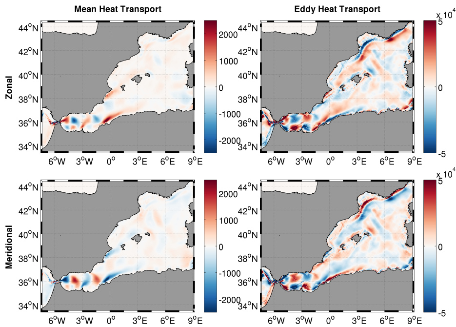
Figure 4.16: Heat transport by mean currents (left) and anomalies (right). The transport is separated into zonal (top) and meridional (bottom) components. The heat transport is given in W \cdot m^{-2}
