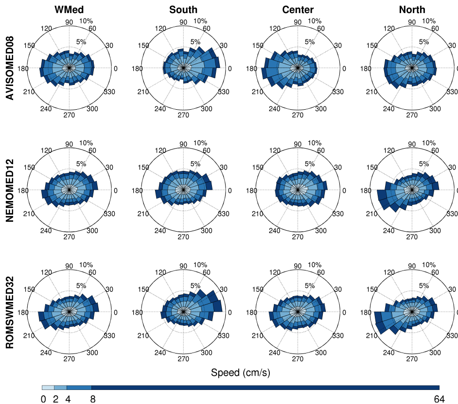
Figure 6.23: Polar histogram of the direction of propagation of the detected eddies. In color is the distribution of velocities in each direction. Eddies from altimetry gridded data are plotted on the first row, eddies from NEMOMED12 on the second row and eddies from ROMS are on the last row. The eddies presented here are only the ones detected by CHE11. The WMed is separated in three different regions: south (Algerian basins), center (Algero-Provençal basin) and north (Gulf of Lion and Balearic Sea).
