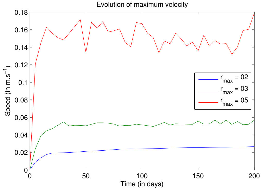
Figure 3.6: Evolution of the maximum velocity in the domain for different topographical smoothing in PGEROMS. Values of r_{x0(max)} tested are 0.2 (blue), 0.3 (green) and 0.5 (red).
