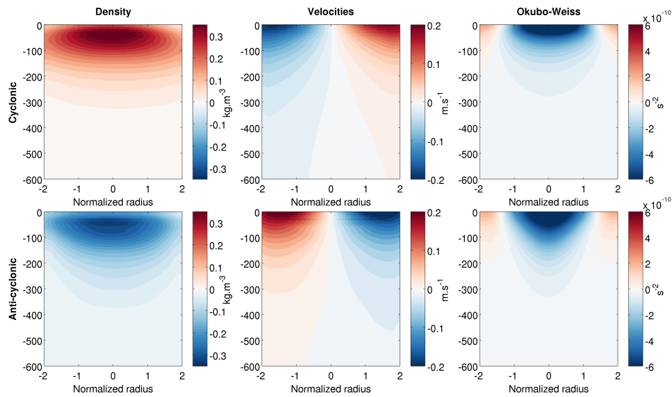
Figure 6.29: Composites of the zonal section of the detected eddies for the anomaly of density, of meridional velocities and the Okubo-Weiss parameter. The density and velocity composites are the mean of anomalies with respect to the climatology. Cyclones are pictured in the first row and anticyclones in the second row. The y-axis of the plots is the depth while the x-axis is a dimensionless distance from the center.
