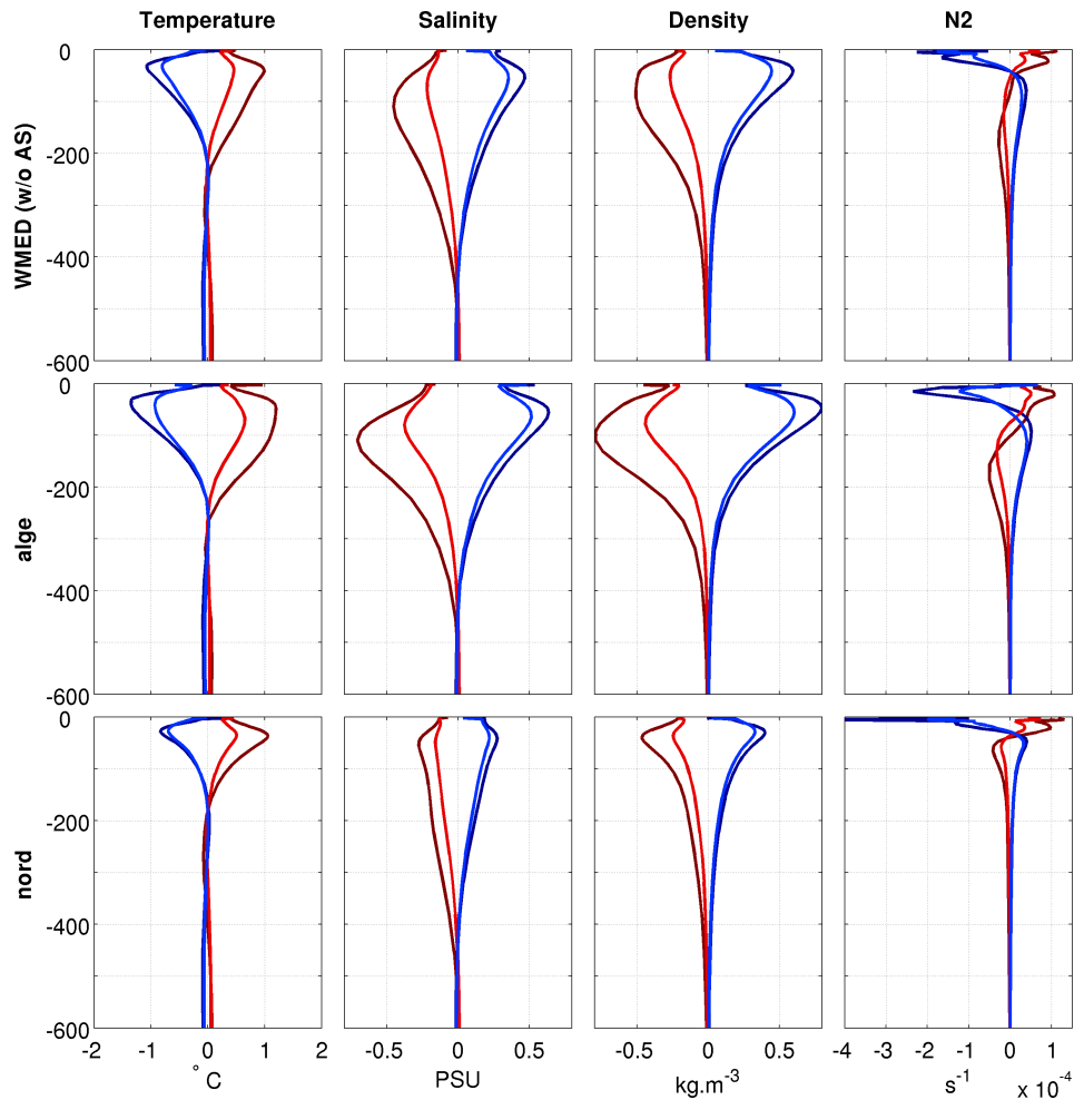
Figure 6.28: Composites of different characteristics (temperature, salinity, density and Brunt-Vaisala frequency) taken in the center of each eddies in the different regions. These composites are the mean of anomalies with respect to climatology of the profiles in the center of the eddies. Cyclonic eddies are in blue and anticyclonic eddies are in red. Darker colors are for long-lived eddies and brighter colors are for short-lived eddies.
