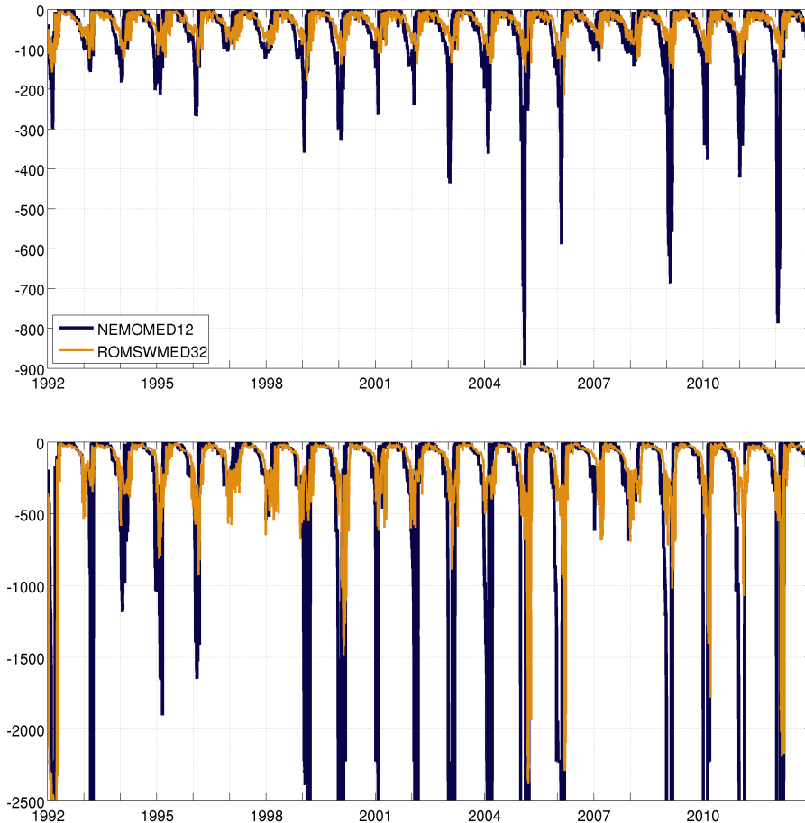
Figure 4.10: Time evolution of the spatially averaged (top) and maximum (bottom) mixed layer depth in the Gulf of Lion for NEMOMED12 in blue and the ROMS simulation in yellow.
