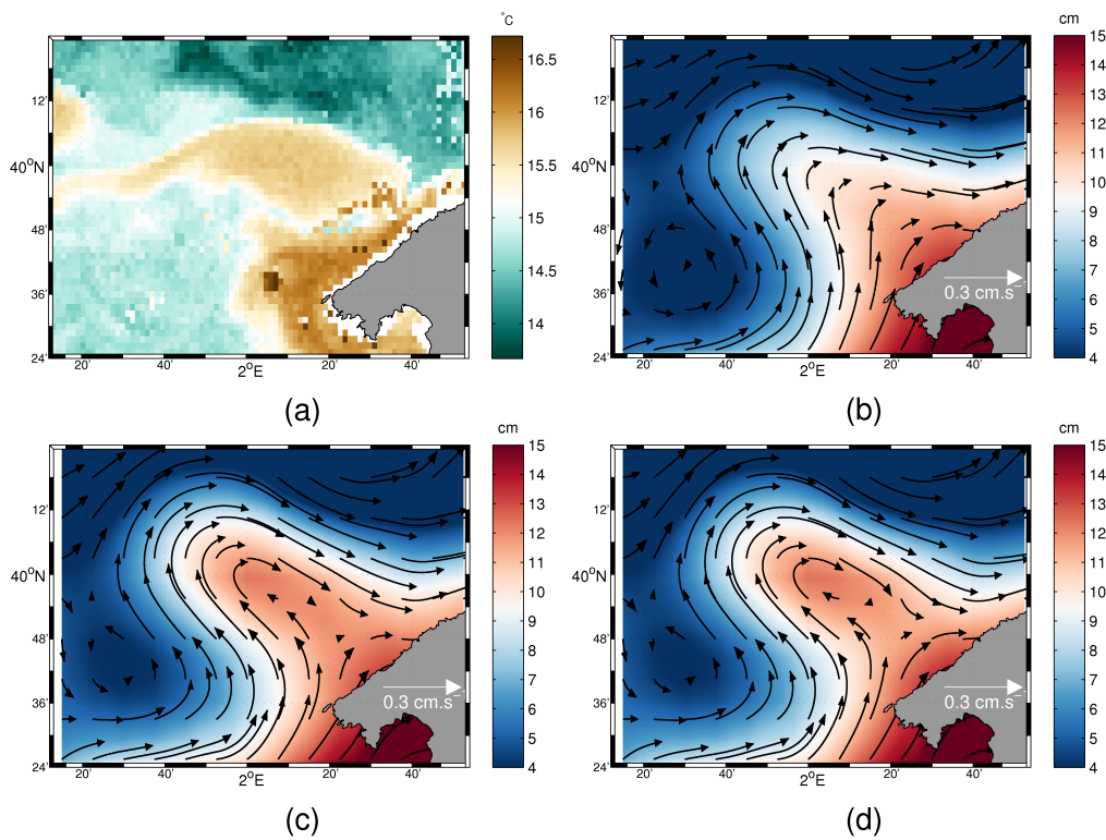
Figure 5.2: (a) Satellite sea surface temperatures (SSTs) on 5 December 2010 for the area north of Mallorca, which were obtained through the GODAE High Resolution SST effort (GHRSSST; www.ghrsst-pp.org ). The ADT overlapped by the derived geostrophic currents from the (b) AVISO, (c) HR and (d) HR+bathy fields linearly interpolated on the same date.
