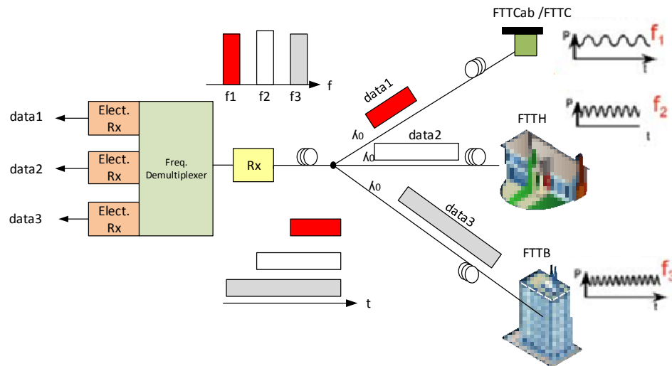
Figure 2.7: Subcarrier Multiple Access
