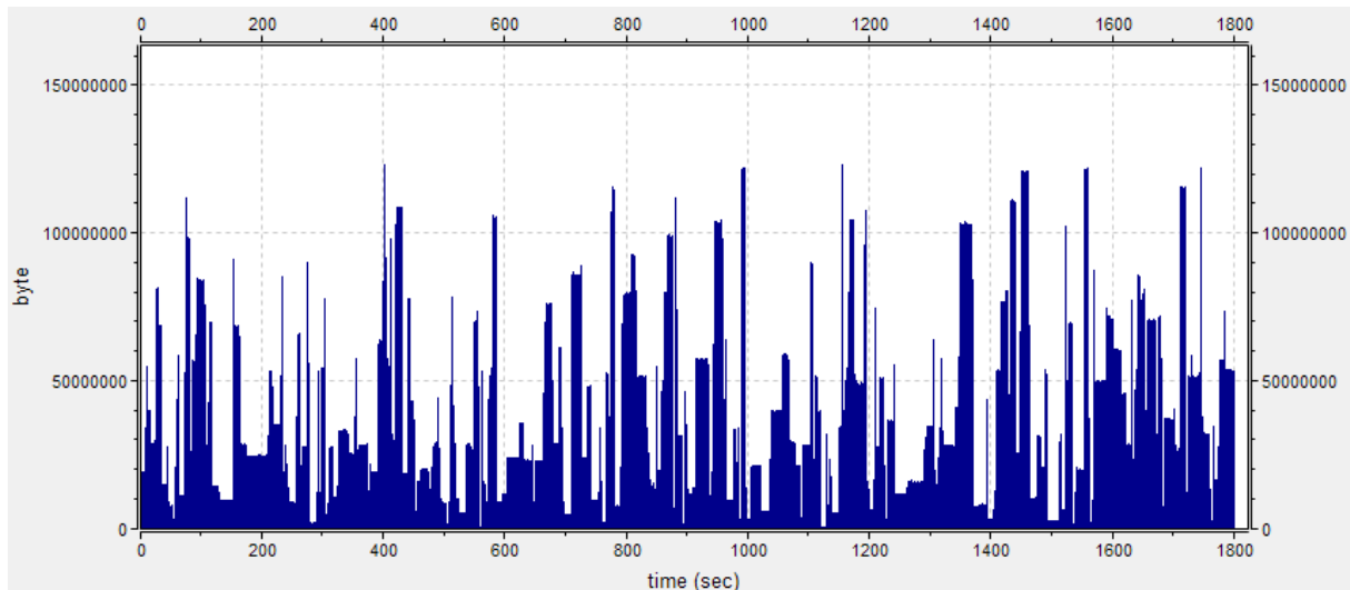
Figure 5.15: Generated traffic example (Average data send – Timeline) 1s intervals, Average Load: 0.38
