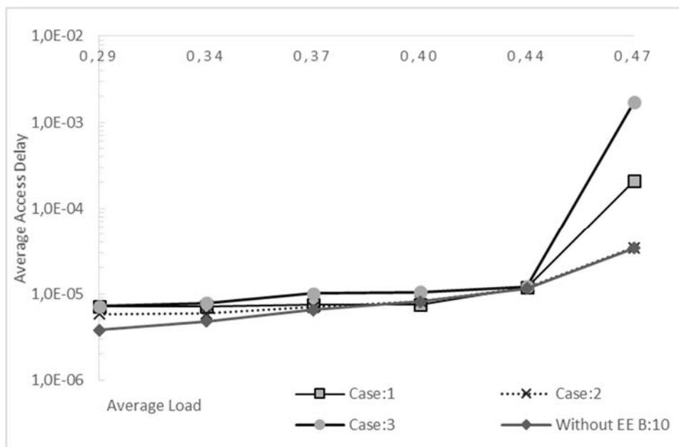
Figure 5.21: Average Access Delay Comparison ( \theta: 10 \text{ sec}, St: 5 \text{ ms}, Rt: 25 \text{ ms} )
