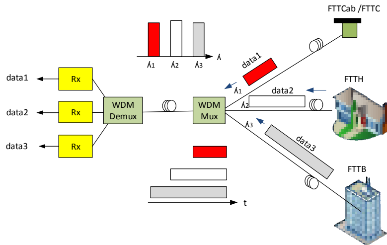
Figure 2.8: Wavelength Division Multiple Access
