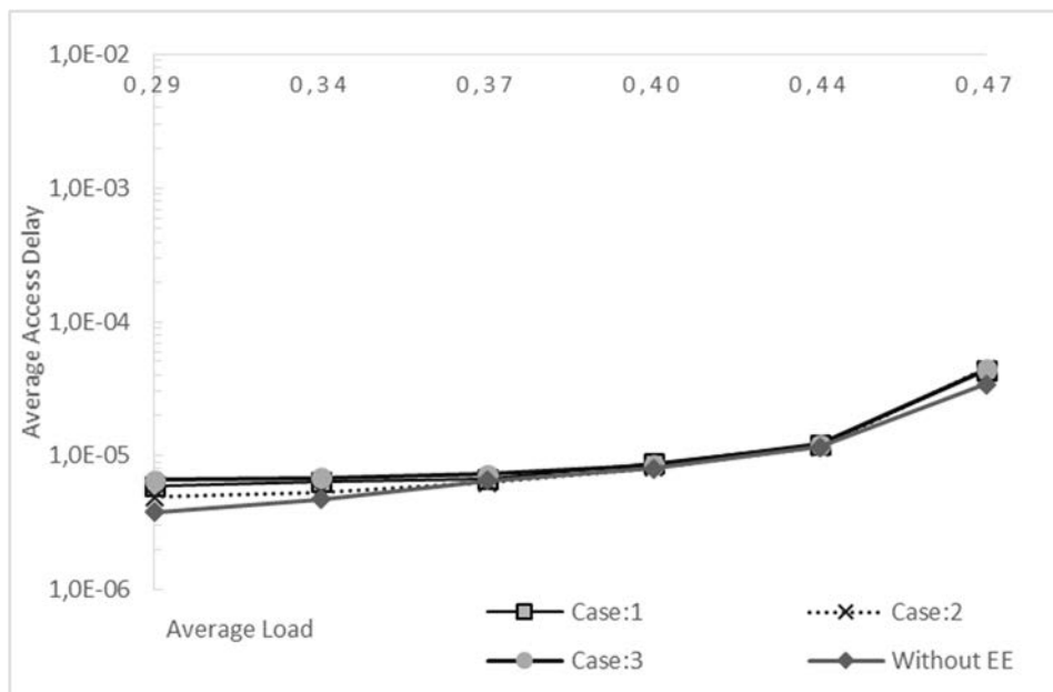
Figure 5.23: Average Access Delay Comparison ( \theta: 10\text{sec}, St: 5\text{ns}, Rt: 5\text{ms} )
