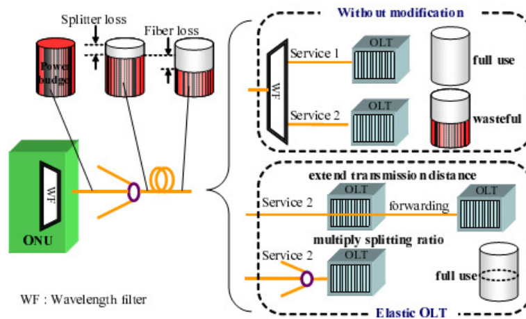
Figure 5.8: Concept of Elastic OLT (Iiyama, et al., 2010)
