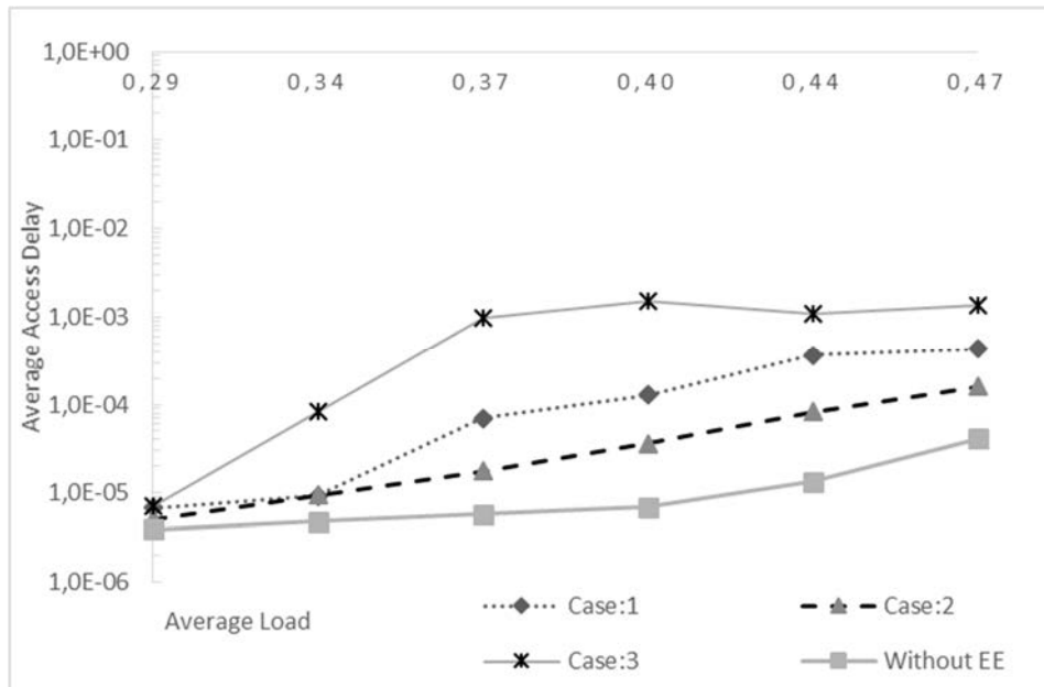
Figure 5.22: Average Access Delay Comparison ( \theta: 3\text{sec}, St: 5\text{ns}, Rt: 5\text{ms} )
