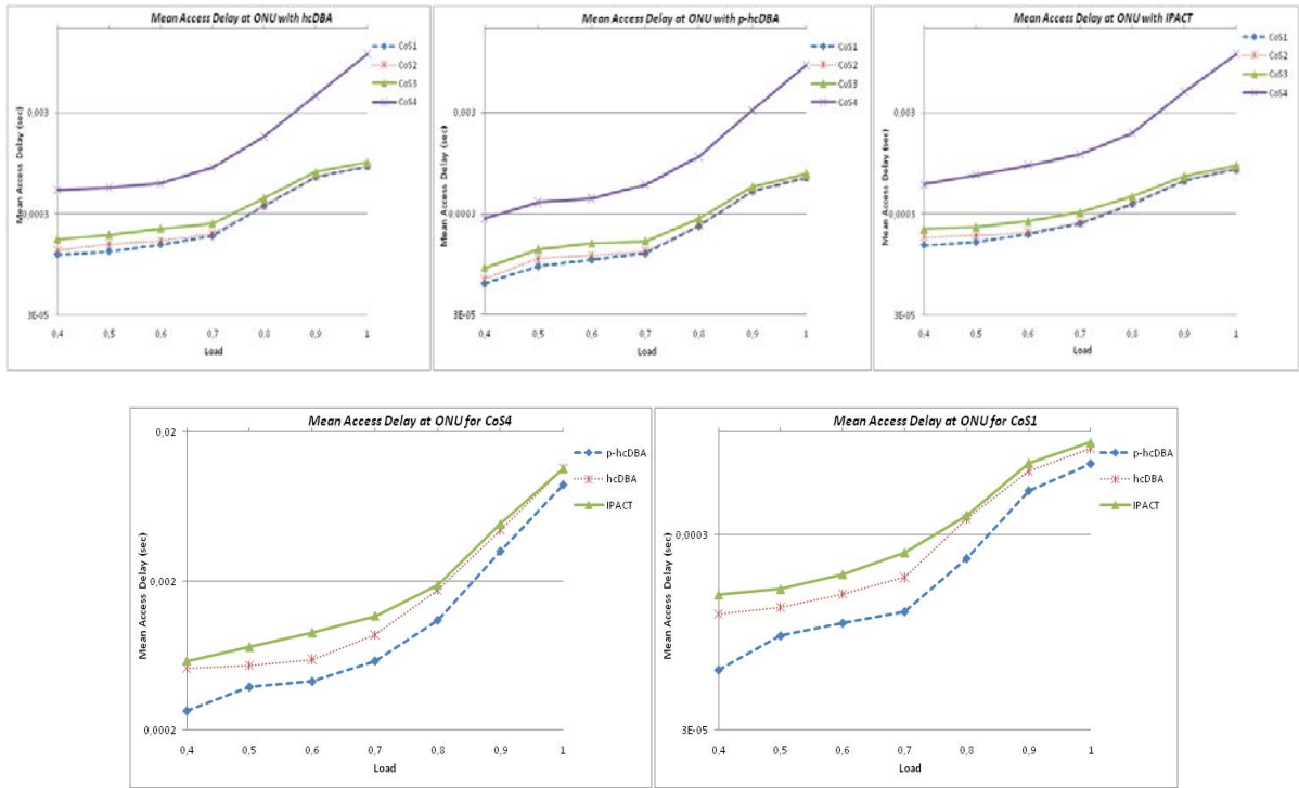
Figure 3.11: Mean Access Delay with Multi-Service Traffic (1 Gbps)
