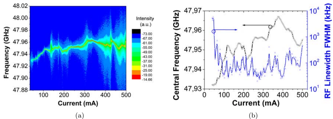
Figure 3.5 – (a) RF spectrum mapping and (b) central frequency and linewidth FWHM evolution as a function of current for the 890\text{-}\mu\text{m} -long single-section QDash MLL at 20 \text{ }^\circ\text{C} .
