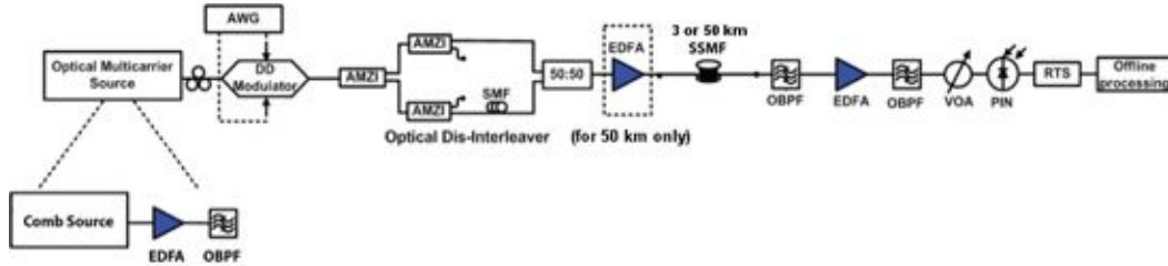
Figure 5.6 – Schematic of the experimental setup for direct detection SSB OFDM transmission (Courtesy of V. Vujicic, DCU).
