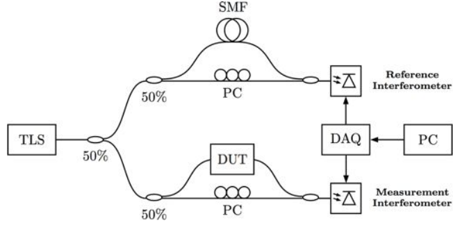
(b) optical frequency-domain interferometry (OFDI)
