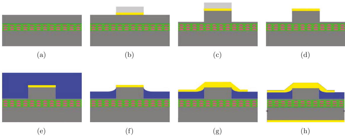
Figure 2.7 – Fabrication steps for shallow ridge waveguide lasers: (a) Deoxidation, (b) etching mask patterning, (c) ridge waveguide etching, (d) etching mask removal, (e) BCB planarization, (f) etching of BCB covering the top of the ridges, (g) deposition of p -type contacts and (h) substrate thinning and deposition of n -type contacts.
