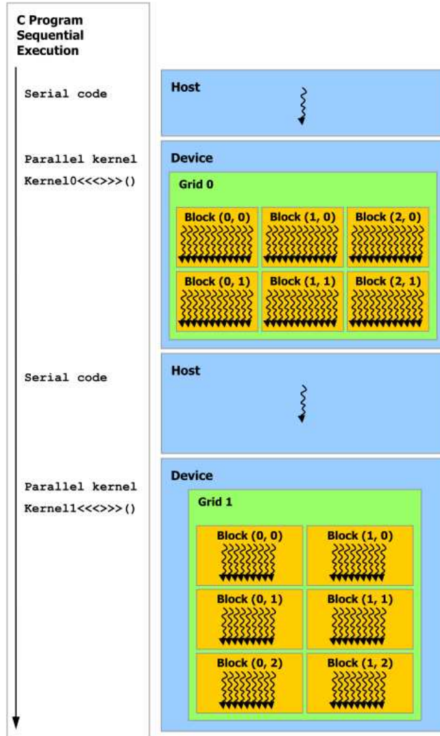
FIGURE 3.14: Heterogeneous Programming.
