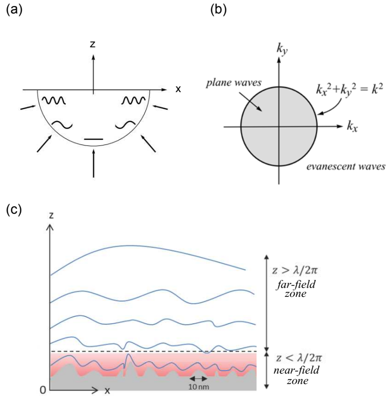
FIGURE 4.1: (a) Illustration of the transverse spatial frequencies of plane waves incident from different angles. The transverse wavenumber (k_x^2 + k_y^2)^{1/2} depends on the angle of incidence and is limited to the interval [0..k] . (b) The transverse wavenumbers k_x , k_y of plane waves are restricted to a circular area with radius k . Evanescent waves fill the infinite space outside the circle. (c) Schematic representation of the near- and far-field zones above a rough diffracting surface. The boundary between the two regions is only vaguely defined, and it depends on the dominant wavelength \lambda emitted by the source.
