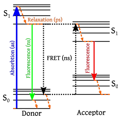
FIGURE 2.10 Jablonski diagram of FRET
