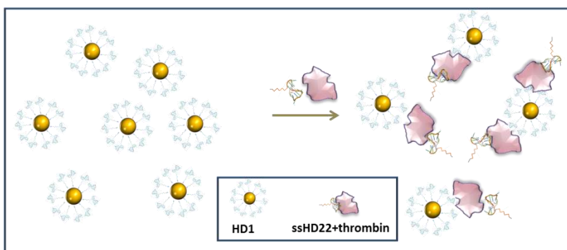
FIGURE 6.5 Interaction of HD1-capped gold nanoparticles in the presence of thrombin-HD22 complex. HD1 interacts only with thrombin exosite I since exosite II is already occupied by stronger aptamer HD22.
