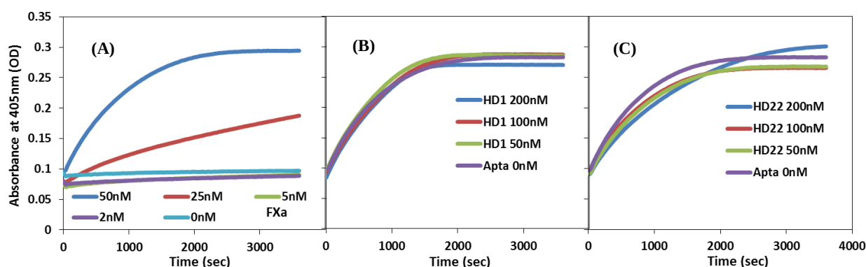
FIGURE 3.14 kinetics of chromogenic substrate cleavage by thrombin activated from 100 nM prothrombin in the presence 2, 5, 25 and 50 nM FXa.(A), or 50 nM FXa and 50, 100, 200 nM HD1 (B) or HD22(C)
