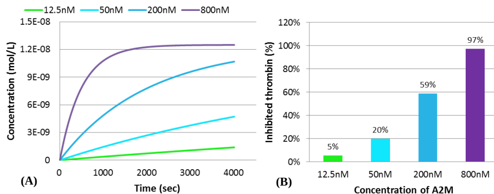
FIGURE 3.29 Inhibition of thrombin by 12.5, 50, 200 and 800 nM A2M. (A) Numerical simulation of 12.5 nM thrombin inhibition by various concentrations of A2M. (B) Concentration of inhibited thrombin after 30 min of incubation with different concentrations of A2M, predicted by numerical simulation.
