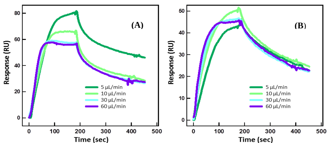
FIGURE 3.5 Determination an optimal flow rate for kinetic experiments. 12.5 nM thrombin was flown over HD1 (A) and HD22 (B) aptamers at 5 ,10, 30 and 60 \mu\text{L}/\text{min} injection rates
