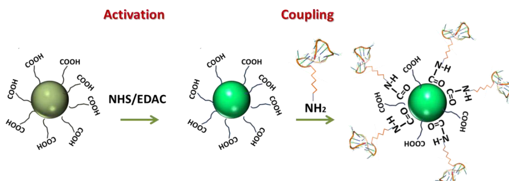
FIGURE 4.6 Schematic illustration of functionalization of carboxyl-modified latex nanoparticles with amino-modified DNA
