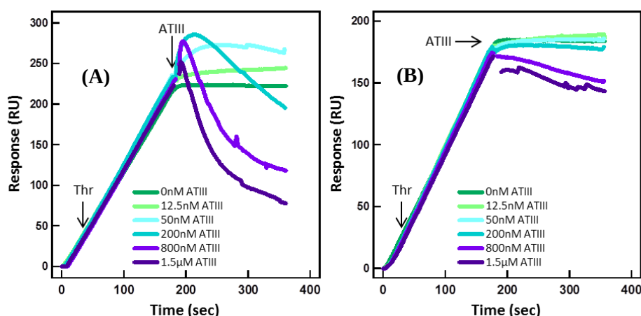
FIGURE 3.22 Sensograms of interaction of various concentrations of ATIII with 12.5 nM thrombin bound to immobilized HD1(A) and HD22 (B) aptamers. First 12.5 nM thrombin was flowed over the densely immobilized aptamers for 3 minutes and then right away increasing concentrations of ATIII were injected.
