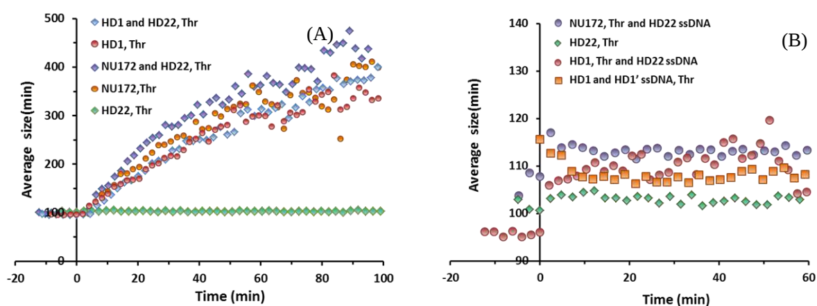
FIGURE 6.3 Measurement of an average hydrodynamic diameter of 80 nm size gold particles functionalized with either HD1, HD22 or NU172 aptamers in the presence of thrombin, thrombin-HD22 complex, thrombin and HD1'. (A) Presence of thrombin induces aggregation with almost similar kinetics in the mixture of HD1-AuNP and HD22-AuNP, NU172-AuNP and HD22-AuNP, or only HD1-AuNP and only NU172-AuNP but not for only HD22-AuNP. (B) Thrombin complexed with ssHD22, didn't allow binding of neither HD1 nor NU172 to thrombin exosite II and thus didn't lead to particle aggregation. Presence of thrombin doesn't induce the aggregation of HD1-AuNPs hybridized with complementary HD1'.
