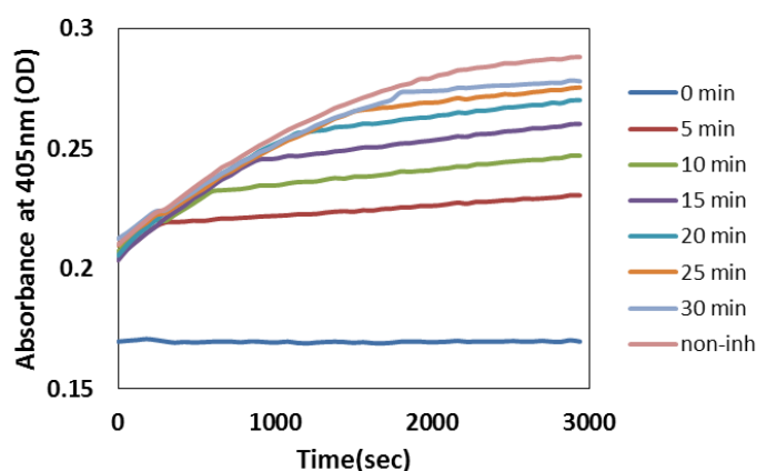
FIGURE 3.15 Kinetics of chromogenic substrate cleavage by thrombin activated from 100 nM Prothrombin with 50 nM FXa. Activity of FXa was inhibited by rivaroxaban each 5 minutes.
