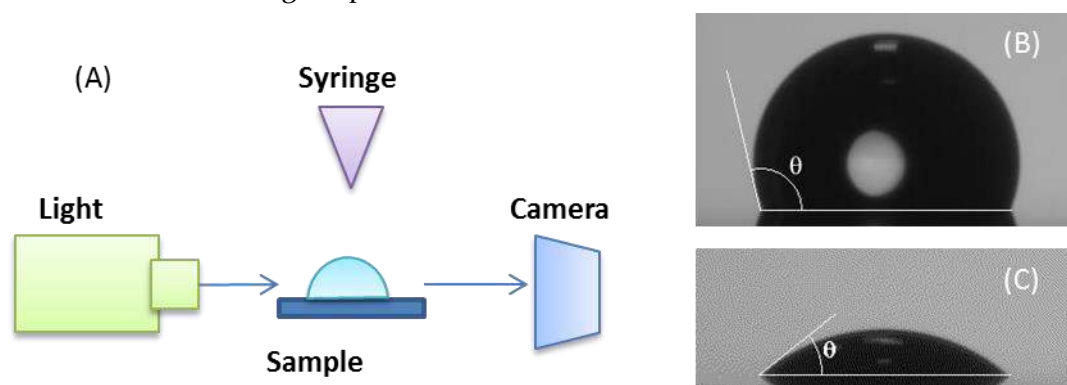
FIGURE 2.13 (A) schematic illustration of the setup for contact angle measurements. Images of the water drop on hydrophobic (B) and hydrophilic surfaces (C).
