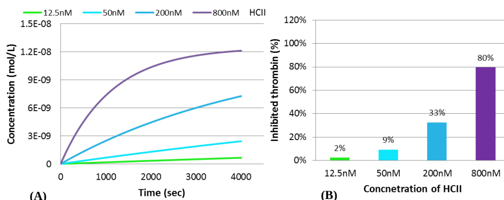
FIGURE 3.25 Inhibition of thrombin by 12.5, 50, 200 and 800 nM HCII. (A) Numerical simulation of 12.5 nM thrombin inhibition by various concentrations of HCII. (B) Concentration of inhibited thrombin after 30 minutes of incubation with different concentrations of HCII, predicted by numerical simulation.
