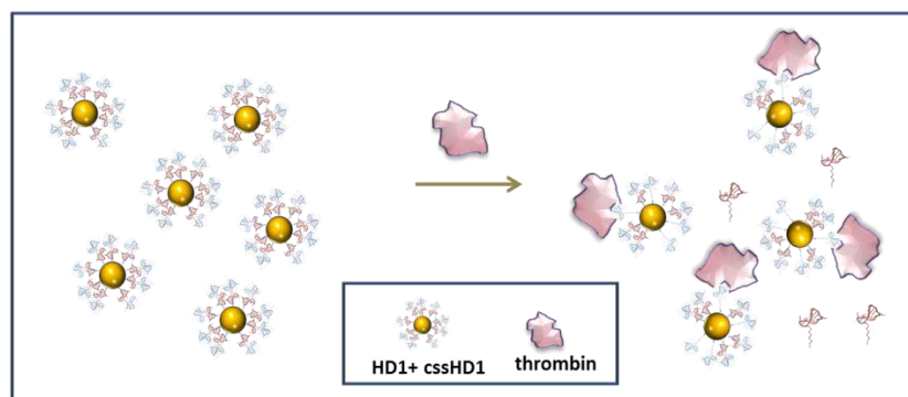
FIGURE 6.6 Interaction of gold nanoparticles bearing HD1 aptamer hybridized to its complementary strand with thrombin. Thrombin exosite I displaces complementary strand and binds HD1 but exosite II being energetically less favorable for binding than complementary strand, remains unbound.
