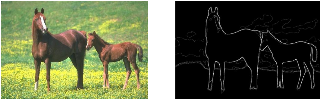
Figure 7.2: Image Segmentation
