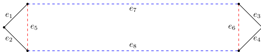
Figure 10.1: In the example, G consists of the edges e_1, \dots, e_8 and R = \{e_1, e_2, e_3, e_4\} . Suppose that e_7 and e_8 have much higher weights compared with e_5 and e_6 . Then the optimal two-edge-connected augmentation would be \{e_5, e_6\} . However, any Steiner tree connecting the edges of R must include one of the edges e_7 and e_8 .
