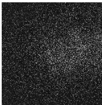
(a) source J1841
