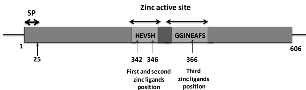
Figure 4: The amino acid sequence of a thermolysin-like metalloprotease (606 aa) from V. tubiashii 07/118 T2. The consensus zinc-binding motif is highlighted in light gray. SP: signal peptide.
