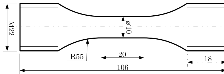
Fig. 1.8: Geometry of CTIF/ENSMA specimens (dimensions in millimetres).
