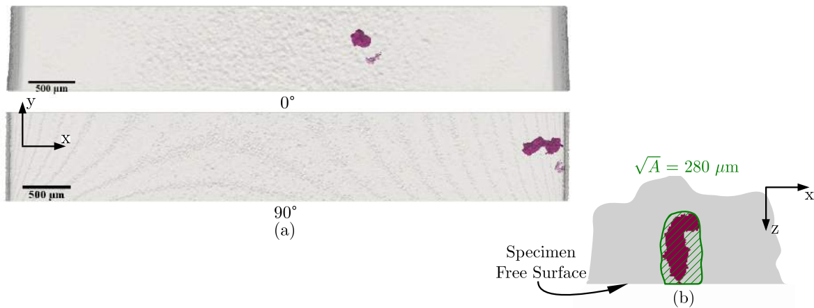
Fig. 2.22: (a) Sample B 3D rendering (voxel size = 6 \mu\text{m} ) of the post-mortem specimen gage at 0^\circ and 90^\circ . (b) Detail of the pore corresponding to the Y projection of the pore. An approximate area projection of the pore is shown in green ( \sqrt{A} = 280 \mu\text{m} ).
