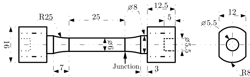
Fig. 1.10: Geometry of torsion specimens (dimensions in millimetres).
