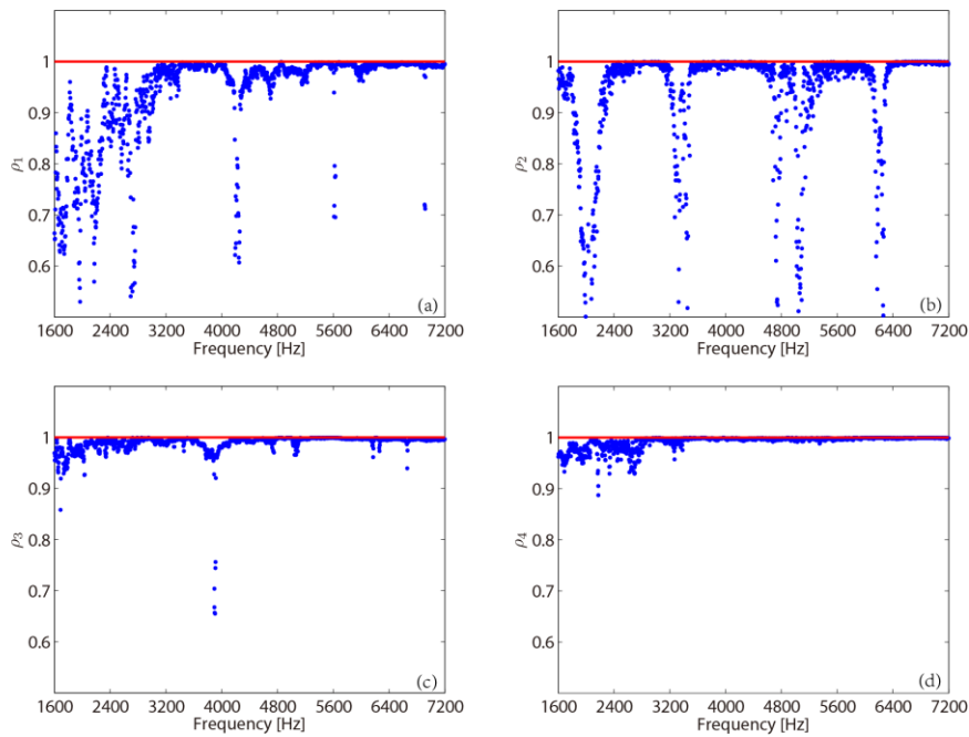
Fig. 6.29 Spatial correlation spectra between the separated and actual sources, \rho_i(\omega) , i = 1, \dots, 4 , from joint approximate diagonalization (blue point) compared to actual sources (red solid line), in the far-field.
