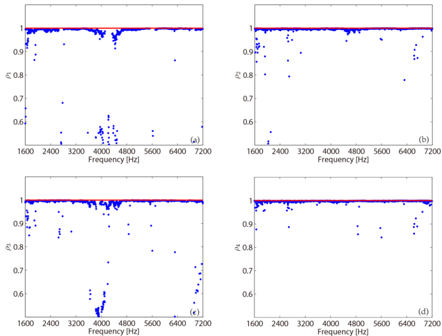
Fig. 6.47 Spatial correlation spectra between the separated and actual sources, \rho_i(\omega) , i = 1, \dots, 4 , from the criterion of least spatial variance, in the far-field.
