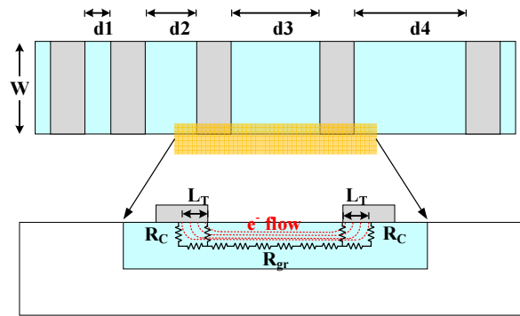
Fig III-25: Schematic of TLM structure.
