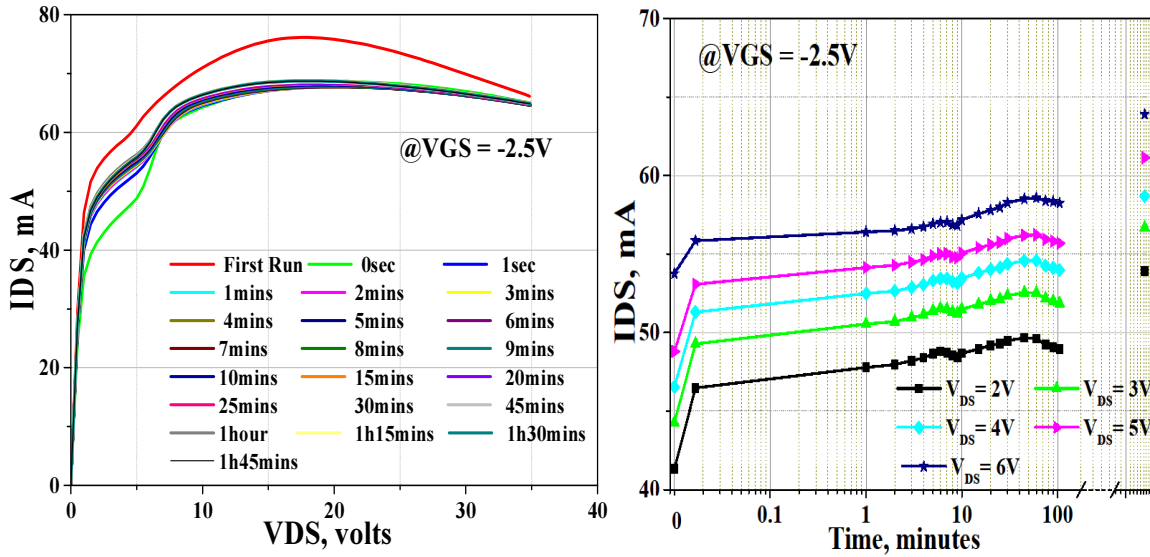
Fig II-17: DC I-V drain curves at V_{GS} = -2.5V at different time interval (a), and time delay to recover initial current value of first run (b)
