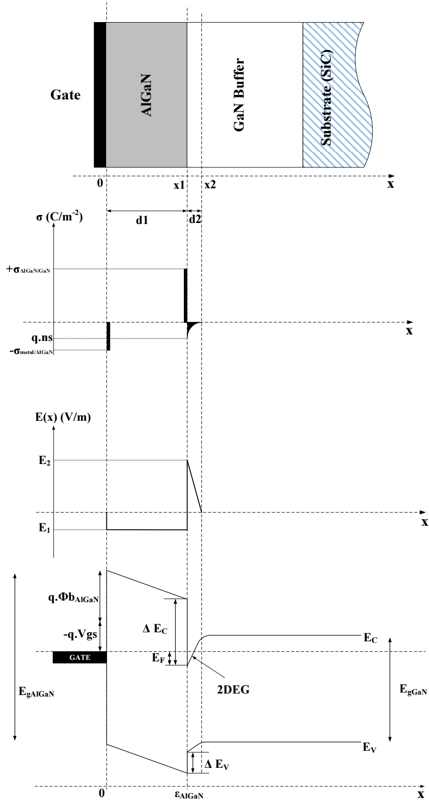
Fig II-5: Charge distribution, electric field and energy band diagram of an AlGaN/GaN HEMT heterostructure [16].
