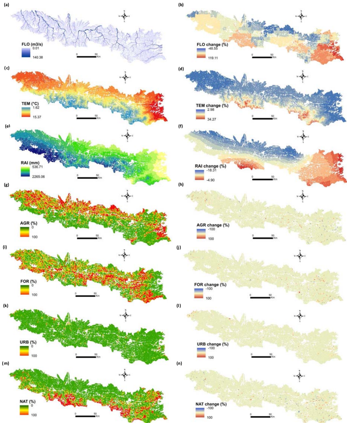
Figure S4. Environmental variables for the historical period (left-hand) and percentage of change over the study period (right-hand): (a, b) stream flow, (c, d) temperature, (e, f) rainfall, (g, h) proportion of agricultural lands, (i, j) proportion of forests, (k, l) proportion of urban areas, and (m, n) proportion of open areas. For the maps showing the percentage of change, a negative value indicates that the current value is lower than the historical value whereas a positive value indicates that the current value is higher than the historical value.
