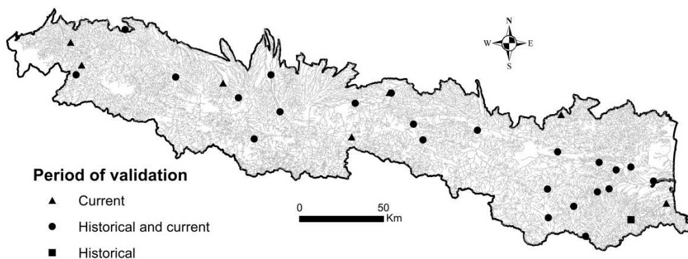
Figure S2. Location of the gauging stations used to calibrate and validate SWAT simulations. They were selected in order to be evenly spatially distributed over the study area, located downstream to have large drainage surface and also according to the accuracy of data measured.
