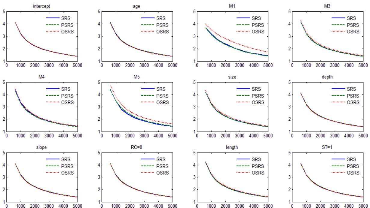
Figure 6-7: the ratio of the average standard errors of simulations divided by the true standard error from population (vertical) versus the calibration sample size (horizontal). Where M1: Brick, M2: vitrified clay, M3: clay tile, M4: reinforced concrete, M5: concrete, RC : road class, ST : sewer type (1 : combined).
