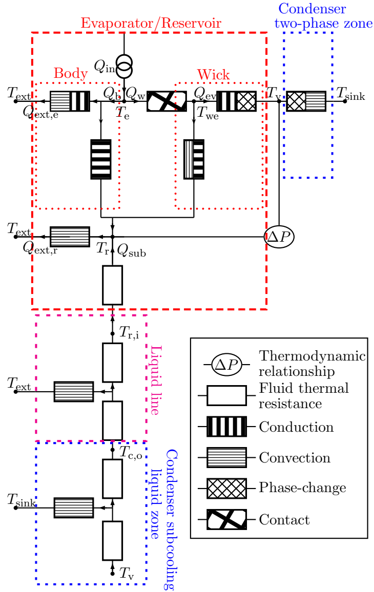
Figure 2.1: LHP schematic nodal network
