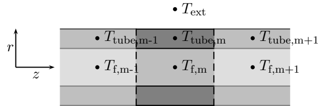
Figure 4.1: Transport lines discretization
