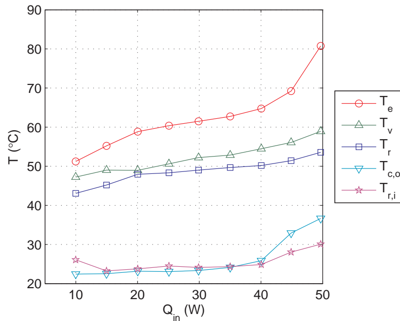
Figure 3.16: Characteristic curve
