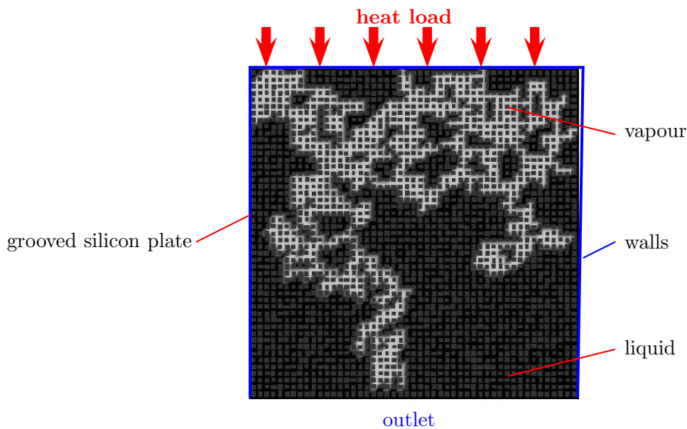
Figure 1.40: Study of the growth of a vapour region inside a porous medium [125]
