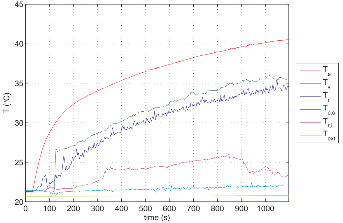
Figure 3.14: start-up of the LHP – Q_{\text{in}} = 10 W
