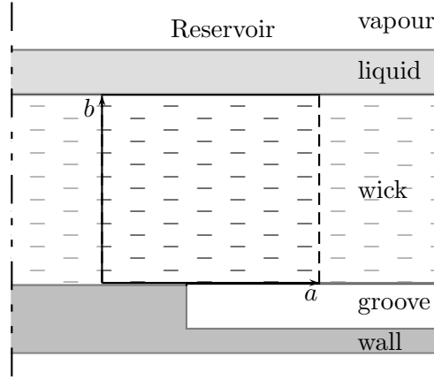
Figure 2.2: Evaporator cross-section
