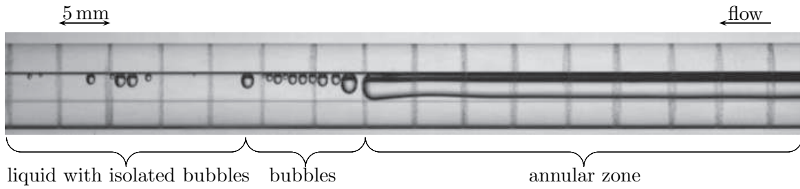
Figure 3.30: Condensation regimes in the condenser – Q_{\text{in}} = 24 \text{ W} , T_{\text{sink}} = 10^\circ\text{C}
