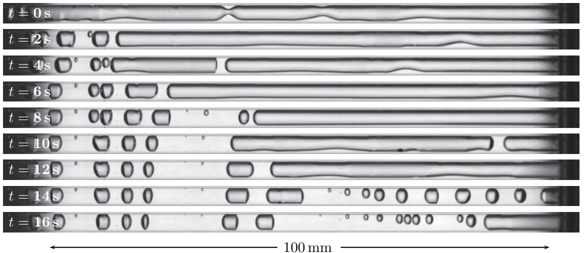
Figure 3.33: Movement of the meniscus in the liquid line – Q_{\text{in}} = 24.8 \text{ W} , T_{\text{sink}} = 30^\circ \text{C}
