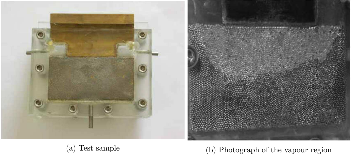
Figure 1.38: Experimental study of a vapour zone development inside a porous structure [124]
