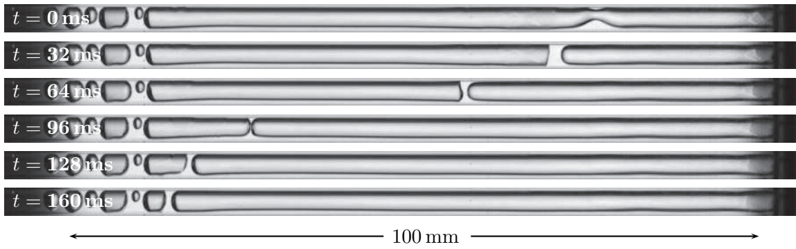
Figure 3.34: Condensation in the liquid line – Q_{\text{in}} = 24.8 \text{ W} , T_{\text{sink}} = 30^\circ \text{C}
