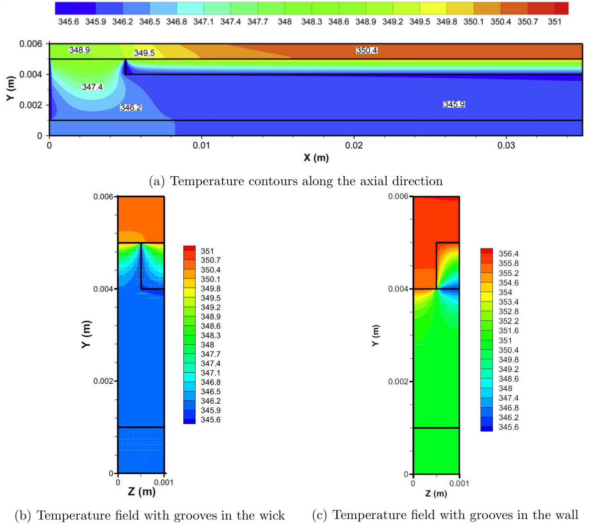
Figure 1.29: Temperature field in the flat evaporator [79]
