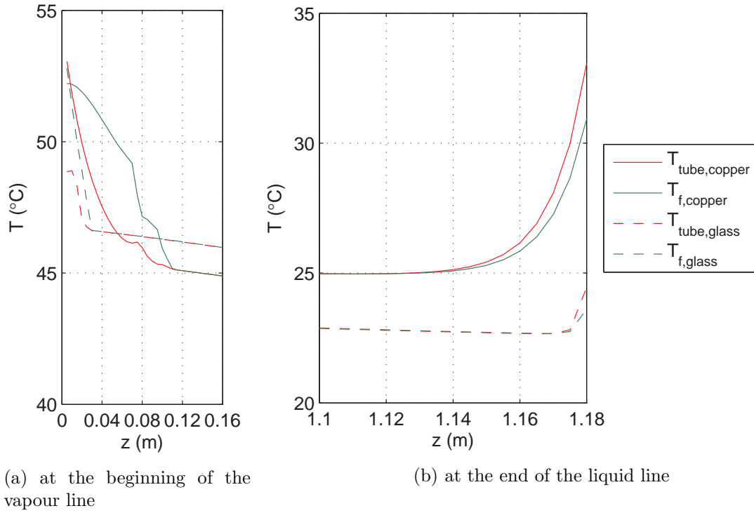
Figure 4.15: Comparison of the temperature profile between the copper tubes (solid lines) and the glass tubes (dashed lines) – Q_{in} = 25 \text{ W}
