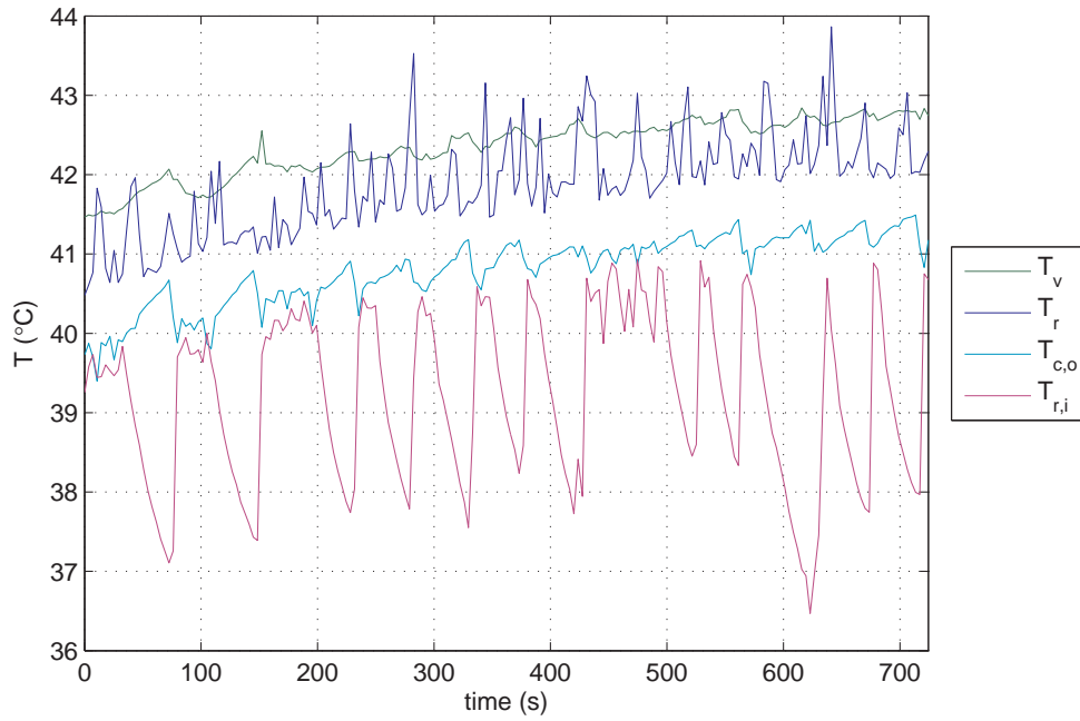
Figure 3.29: Oscillations at the end of the liquid line – Q_{\text{in}} = 20.2 \text{ W} , T_{\text{sink}} = 20^\circ\text{C}
