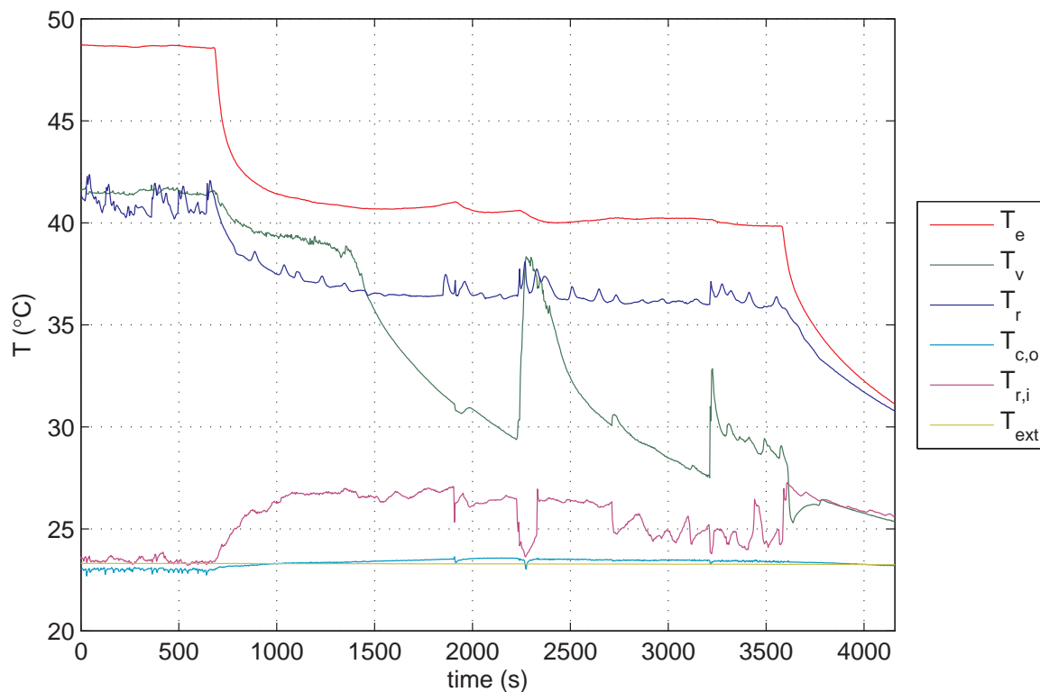
Figure 3.15: Operation at very low heat load – Q_{in} = 5 W
