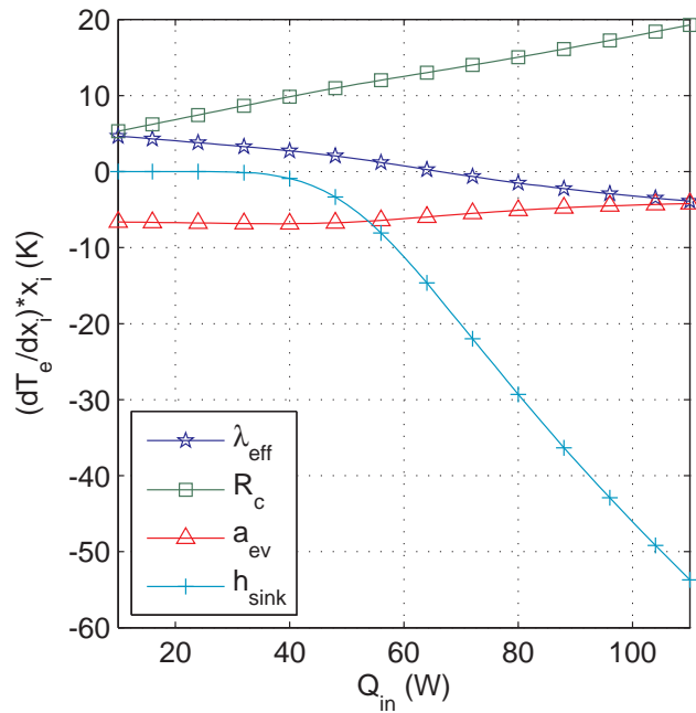
Figure 2.13: Relative sensitivity of T_e to various parameters
