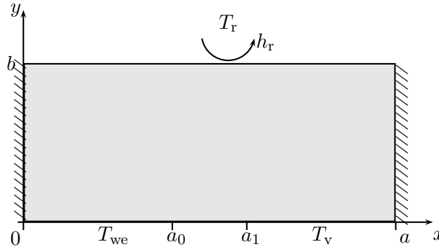
Figure C.1: Schematic of the alternative wick model
