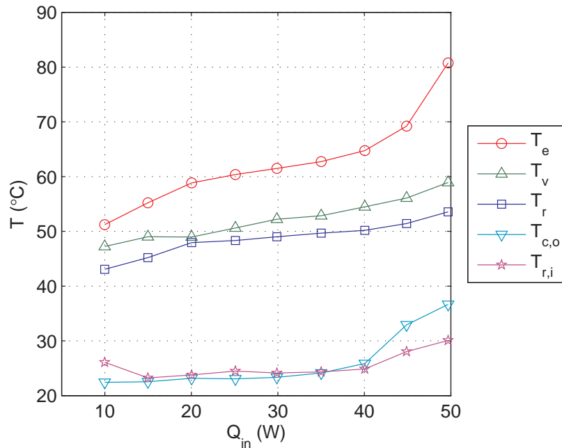
Figure 3.16: Characteristic curve
