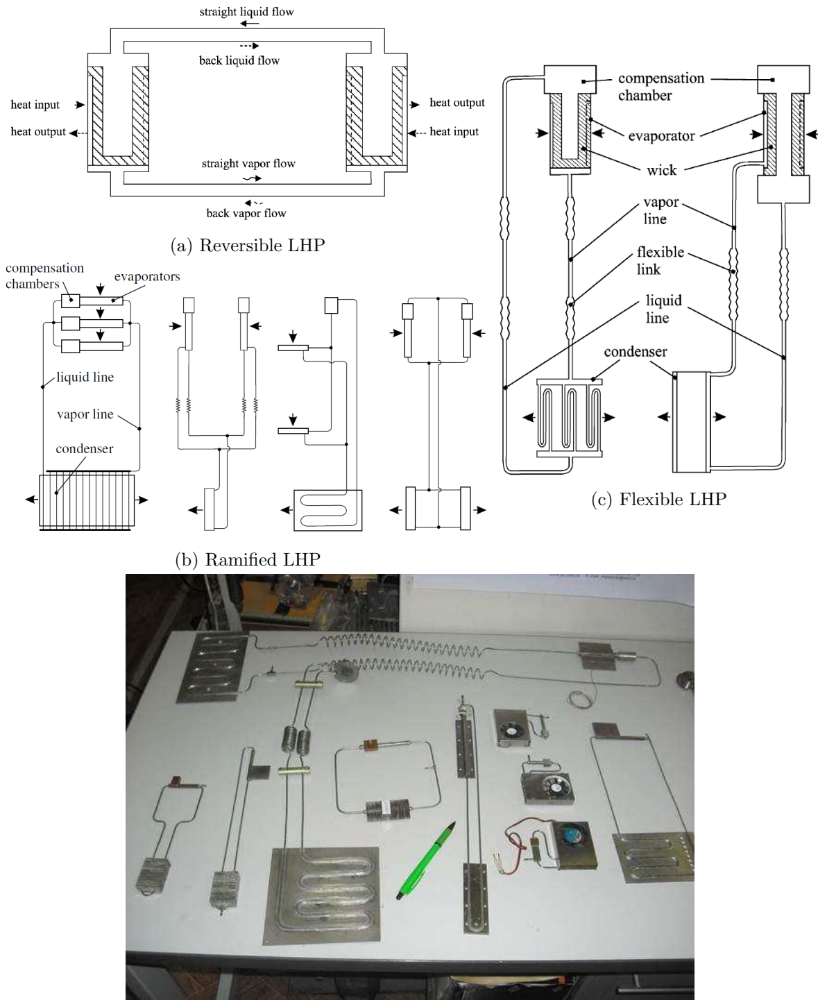
Figure 1.4: Various designs of LHP [20]
