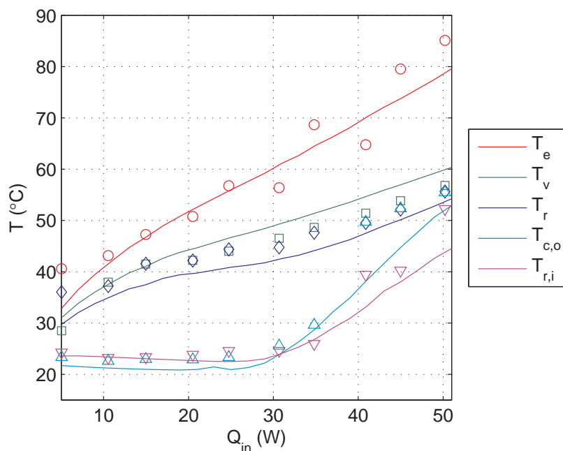
Figure 4.5: Comparison between the numerical simulation and the experimental data: characteristic curve
