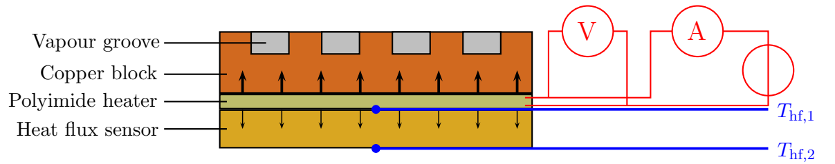
Figure 3.6: Heat input measurement
