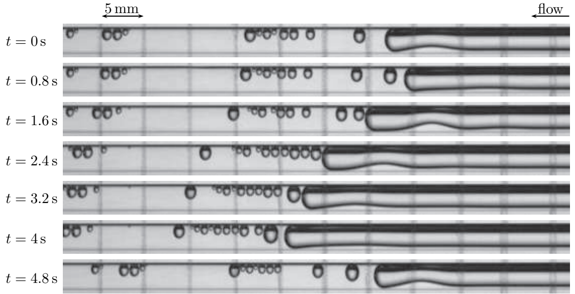
Figure 3.32: Location of the meniscus in the condenser, Q_{\text{in}} = 24 \text{ W} , T_{\text{sink}} = 10^\circ \text{C}
