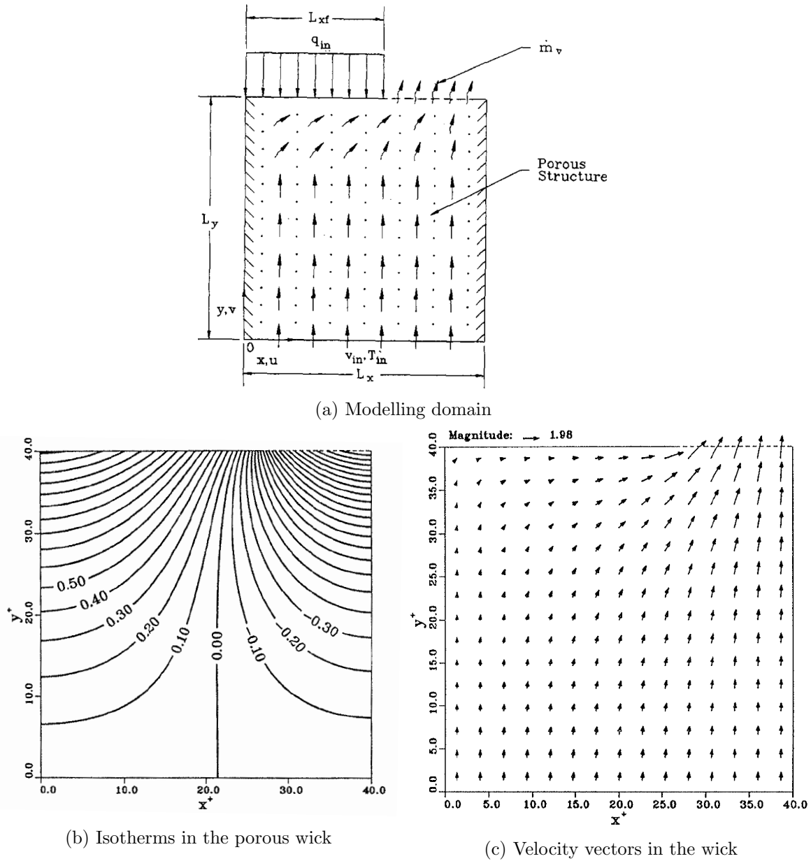
Figure 1.32: Analytical heat and mass transfer in the wick [133]
