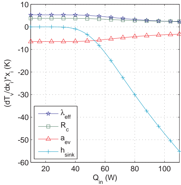
Figure 2.12: Relative sensitivity of T_v to various parameters
