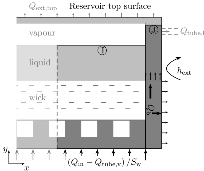
Figure 4.4: Heat transfer to the ambient and through the body
