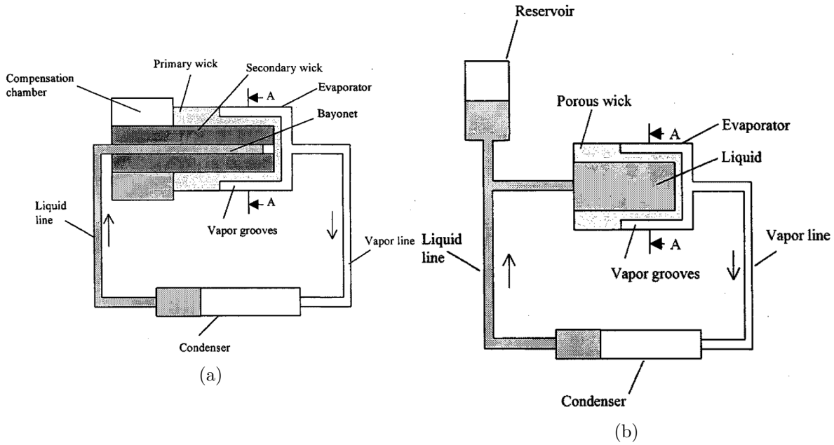
Figure 1.2: Schematic of (a) a traditional LHP and (b) a traditional CPL [10]
