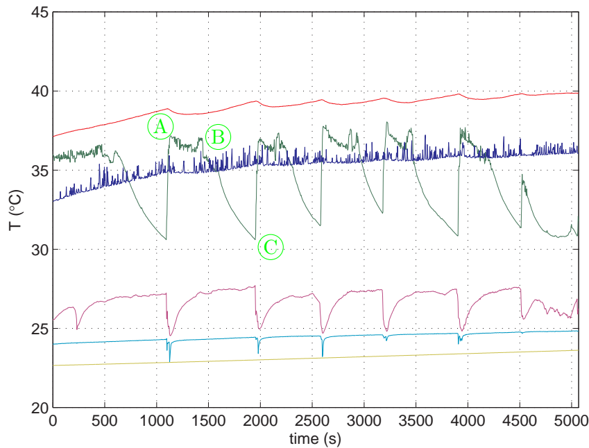
Figure 3.28: Oscillations during a start-up at 5 W – T_{\text{sink}} = 20\text{ }^{\circ}\text{C}
