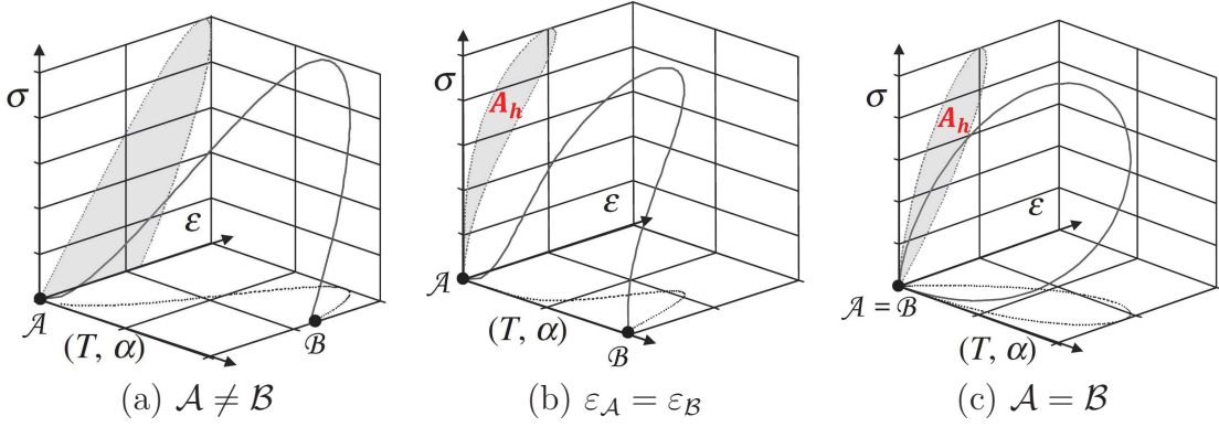
FIGURE 1.3 – Trajets thermomécaniques [Chrysochoos et al. , 2010]
