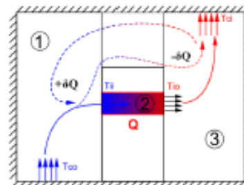
Figure 19: by-pass / recirculation phenomenon
