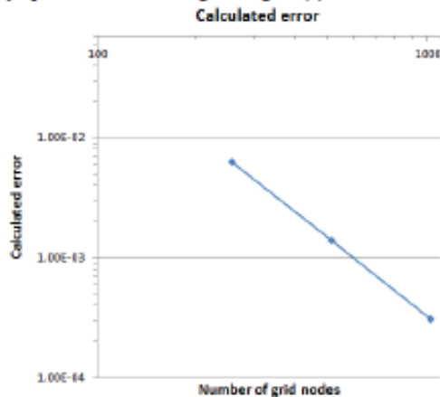
FIGURE 5: Asymptotic zone of convergence
