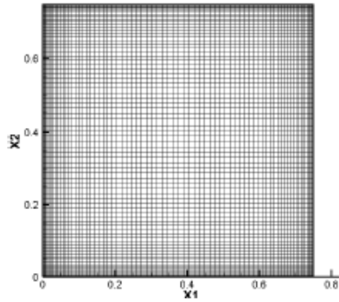
FIGURE 6: 80 \times 80 Chebyshev grid
