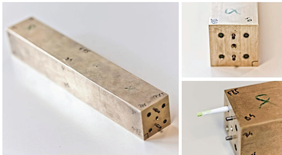
Figure 7.13: Pictures of the brass absorber containing the four LuAG fibers. This CFCAL was inserted among \text{PbWO}_4 crystals in the EE module facing the beam.
