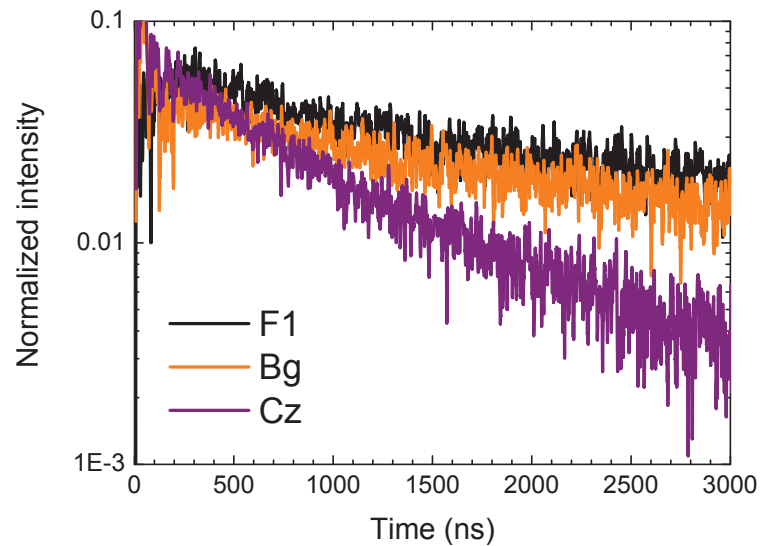
Figure 4.12: Timing profile of the intrinsic scintillation for samples grown by either \mu PD ( F_1 ), Bridgman ( Bg ) or Czochralski ( Cz ) techniques.
