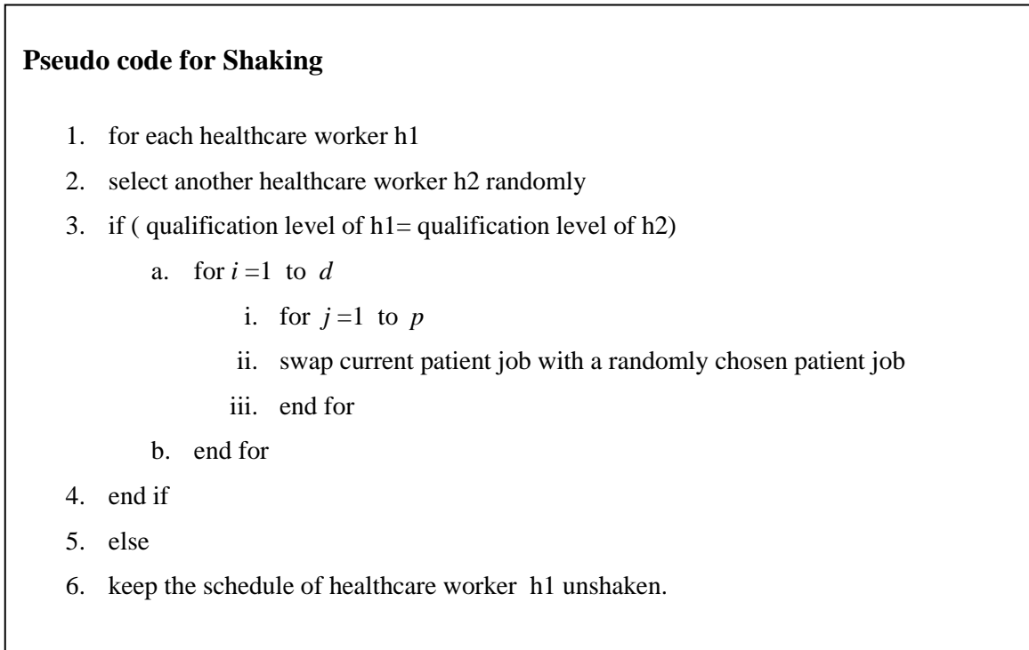
Figure 5.9: Pseudo code for Shaking
