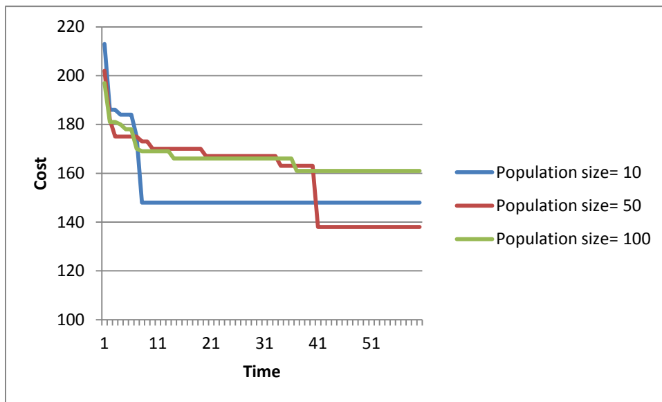
Figure 5.22: Graph representing comparison for different population size on GA algorithm. Here X-axis represents time and Y-axis represents the cost.
