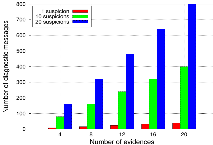
Figure 4.17: Economizing detection messages thanks to confidence interval.
