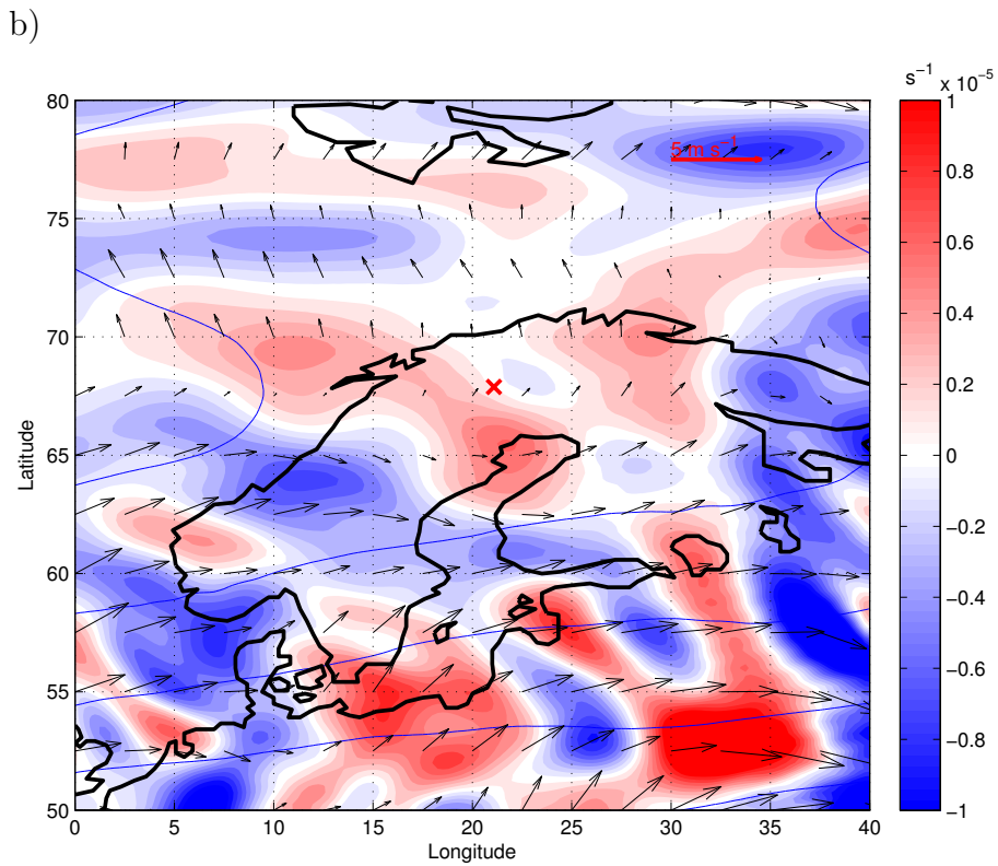
Figure 4.3: Wind field (vectors), geopotential height (blue contours), and relative vorticity (shaded contours) for Case # 1 from the 24 h lead time ECMWF control forecast on 16 August 2009 at 18UTC a) at 500 hPa and b) at 50 hPa. The contour interval for the geopotential height is 25 m. The red cross denotes the launch site.
